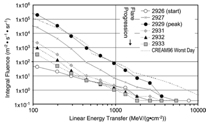
Fig. 22. Comparison of a solar heavy ion event that occurred in November 2001 with the CREM96 “worst day” model. The progression of daily intensities is indicated with the peak intensity occurring on day 2929 of the mission [94].
