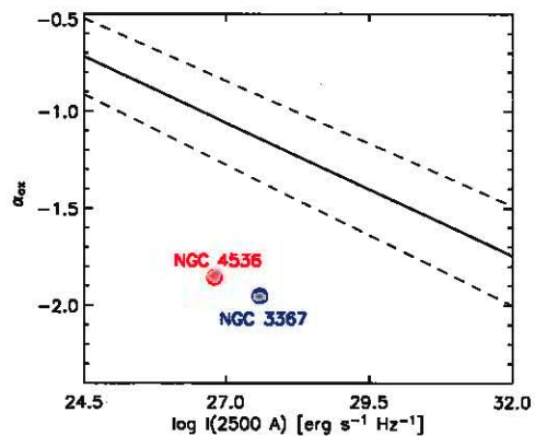
FIG. 4.— \alpha_{OX} plotted versus 2500 Å monochromatic luminosity. The solid line corresponds to the best-fit relation derived by Steffen et al. (2006) and the dashed lines account for the uncertainties in the fit.
