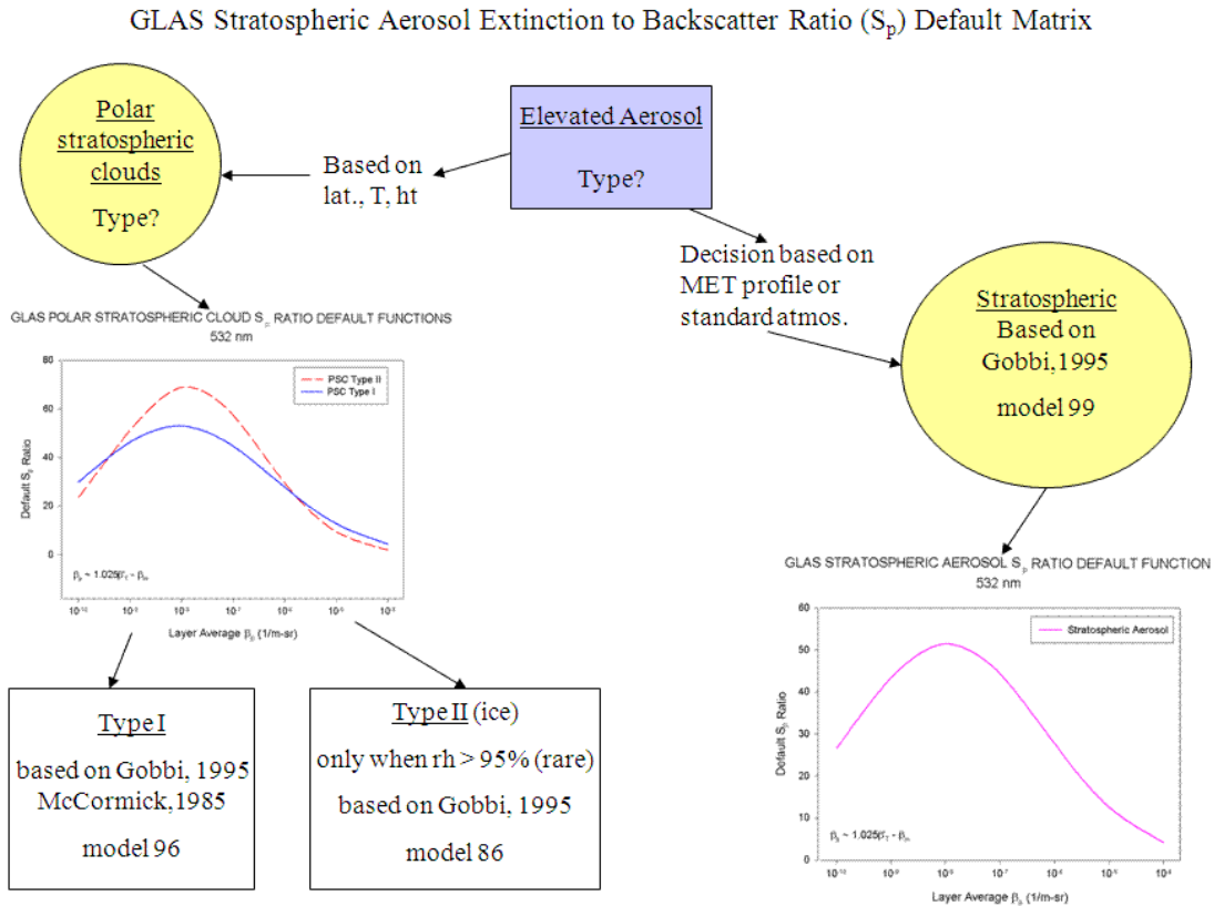
Figure 4.5.1 Flow diagram for GLAS Stratospheric S_p ratio Default Matrix
