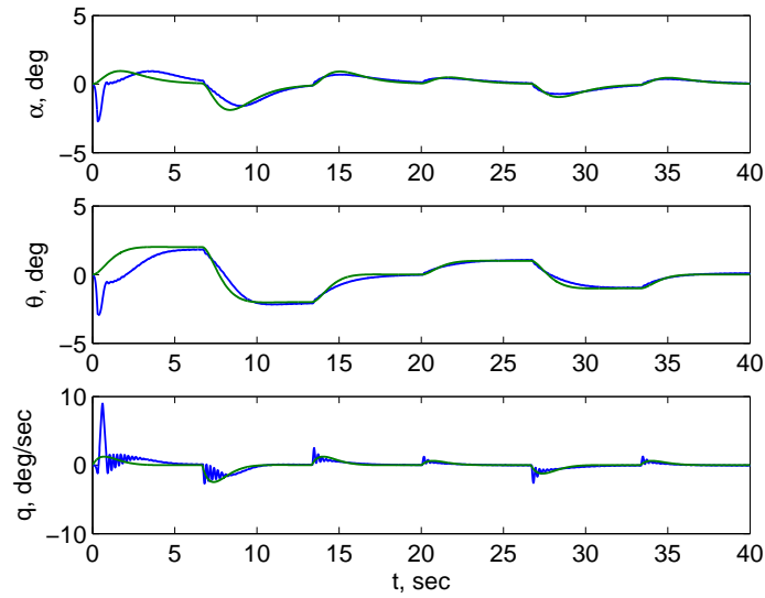
Figure 6 - Stable Aircraft Response with Standard MRAC
