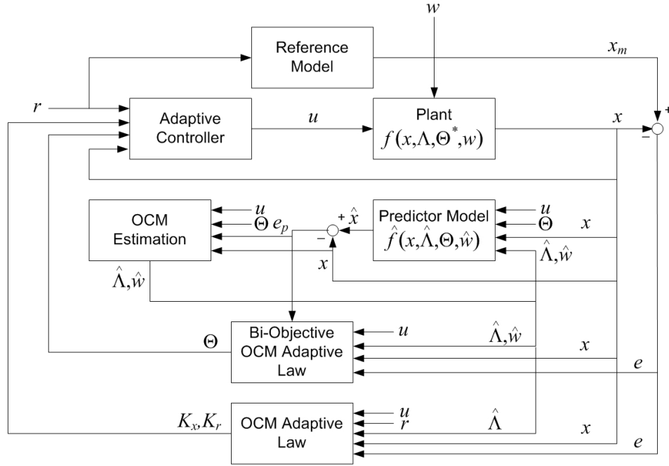
Figure 1 - Adaptive Control Architecture with Bi-Objective Optimal Control Modification
