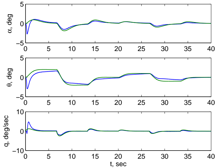
Figure 9 - Stable Aircraft Response with Bi-Objective Optimal Control Modification (OCM)
