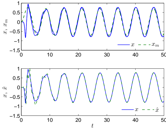
Figure 2 - x(t) , \hat{x}(t) , and x_m(t)
