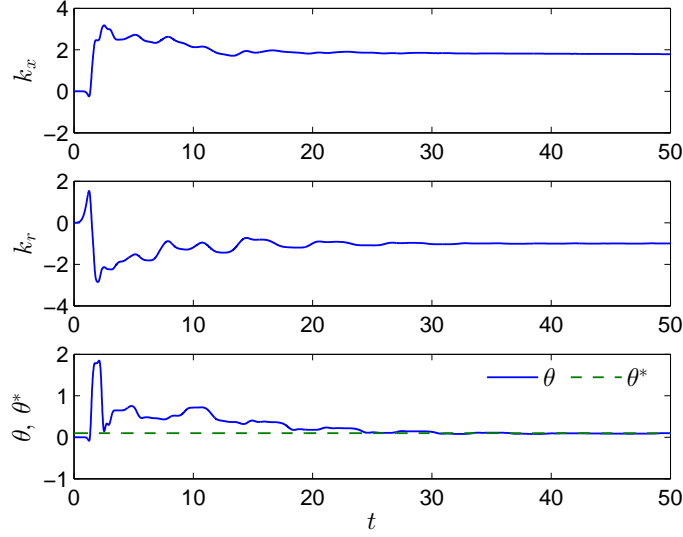
Figure 3 - k_x(t) , k_r(t) , and \theta(t)
