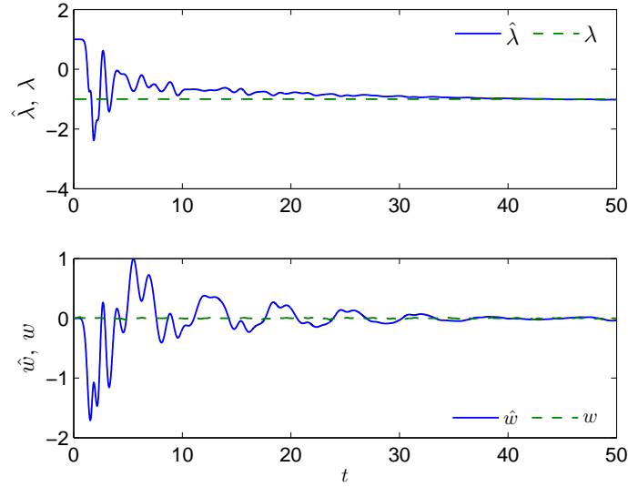
Figure 4 - \hat{\lambda}(t) and \hat{w}(t)
