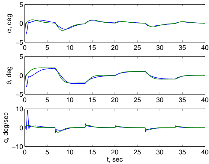
Figure 8 - Stable Aircraft Response with Bi-Objective MRAC \gamma_w = 0
