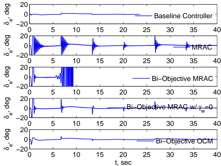
Figure 10 - Elevator Deflections
