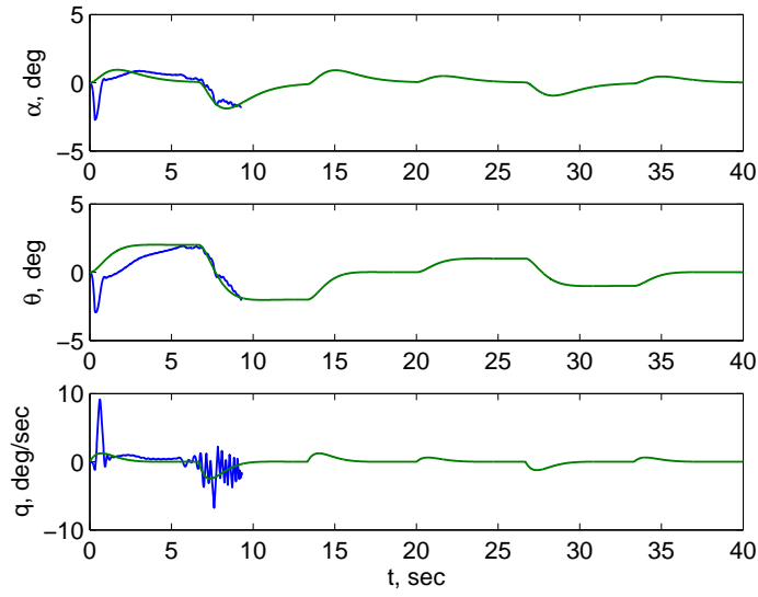
Figure 7 - Unstable Aircraft Response with Bi-Objective MRAC \gamma_w > 0
