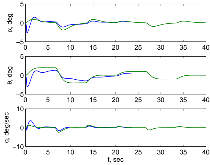
Figure 5 - Unstable Aircraft Response with Baseline Controller
