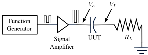
Figure 2. Block diagram of the experimental setup.
