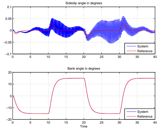
Fig. 4. MRAC angle tracking performance with \gamma = 1000 .
