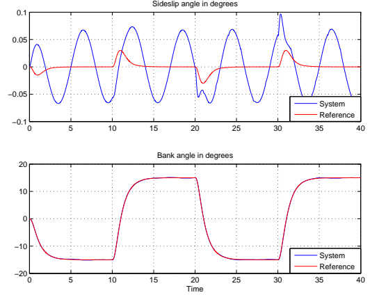
Fig. 1. M-MRAC angle tracking performance with \gamma = 1000 .
