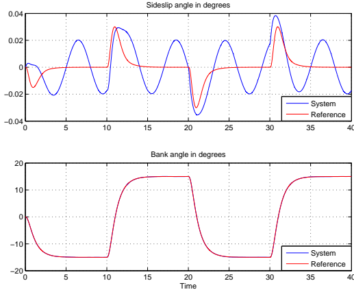
Fig. 7. M-MRAC output tracking with \gamma = 10000 .
