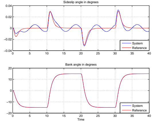
Fig. 9. M-MRAC output tracking with \gamma = 100000 .
