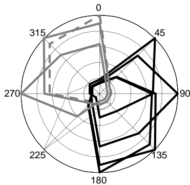
Figure 12. Maximum cross-correlation of pressures at CM-SM junction, M=0.9 , pitch= 0^\circ , roll= 0^\circ , protuberances on.
