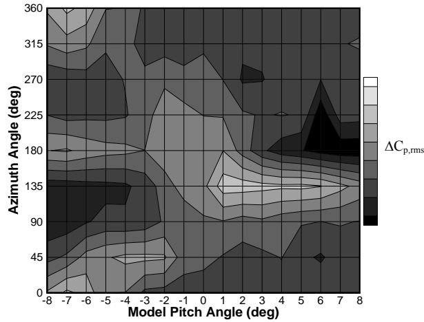
Figure 16. Measured \Delta C_{p,rms} as a function of model pitch angle and transducer azimuthal location, M=0.9 , roll = 0^\circ , protuberances off.
