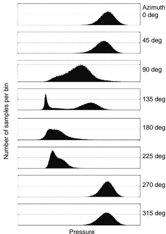
Figure 11. Histogram of pressure time histories at CM-SM junction, M=0.9 , \text{pitch}=4^\circ , \text{roll}=0^\circ , protuberances on.
