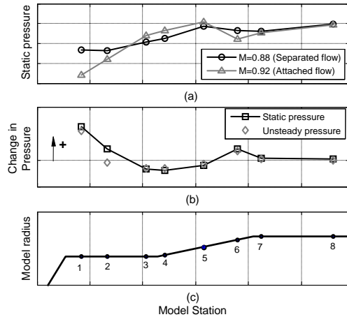
Figure 19. Relationship between static pressures at M=0.88 and 0.92 and the alternating flow pressure amplitude at M=0.9, pitch=0°, roll=0°, protuberance on.
