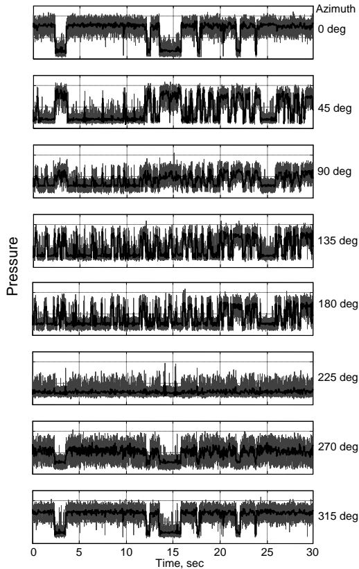
Figure 9. Pressure time histories at CM-SM junction, M=0.9 , \text{pitch}=0^\circ , \text{roll}=0^\circ , protuberances on. Unfiltered time histories (gray), low-pass filtered time histories (black).
