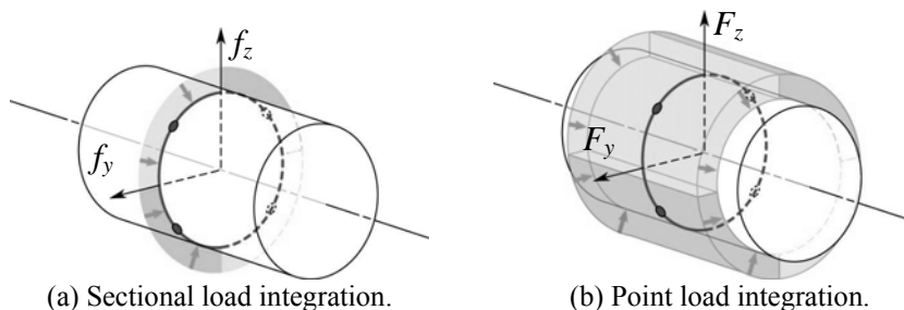
Figure 4. Loads resulting from two methods of pressure integration.
