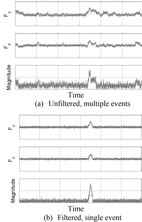
Figure 20. Buffet forcing functions just aft of the expansion corner, M=0.9 , \text{pitch}=1^\circ , \text{roll}=0^\circ , protuberance on.
