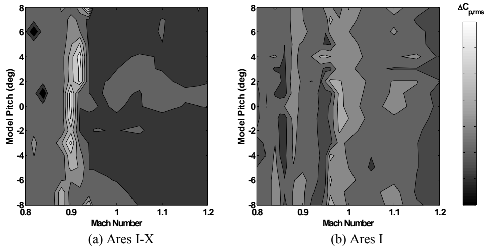
Figure 8. Contour plot of peak \Delta C_{p,rms} versus model pitch and Mach number, protuberances on.
