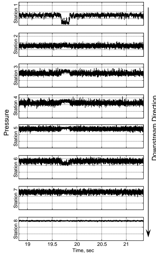
Figure 18. Pressure time histories measured downstream of CM-SM junction at 0 degree azimuth, M=0.9 , pitch= 0^\circ , roll= 0^\circ , protuberance on.
