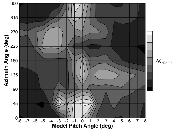
Figure 14. Measured \Delta C_{p,rms} as a function of model pitch angle and transducer azimuthal location, M=0.9 , roll = 0^\circ , protuberances on.
