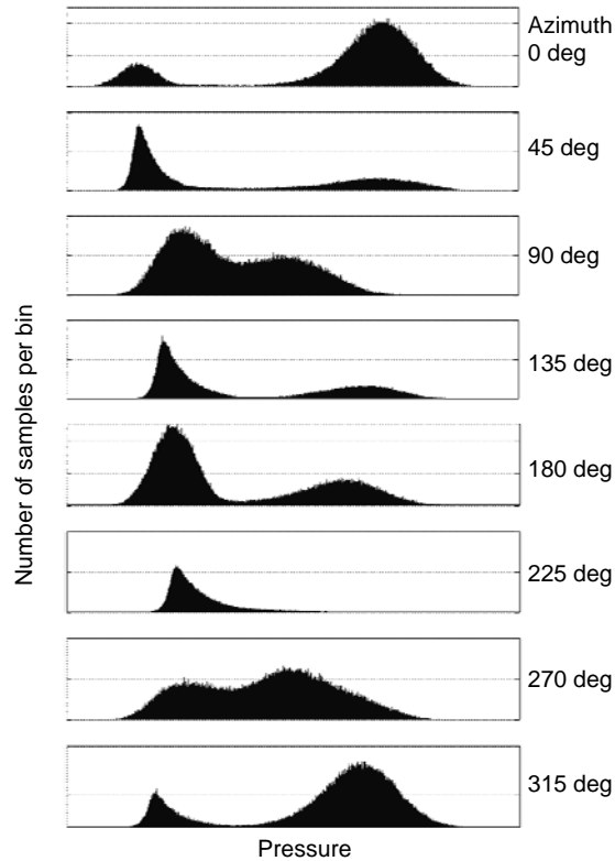
Figure 10. Histogram of pressure time histories at CM-SM junction, M=0.9 , \text{pitch}=0^\circ , \text{roll}=0^\circ , protuberances on.
