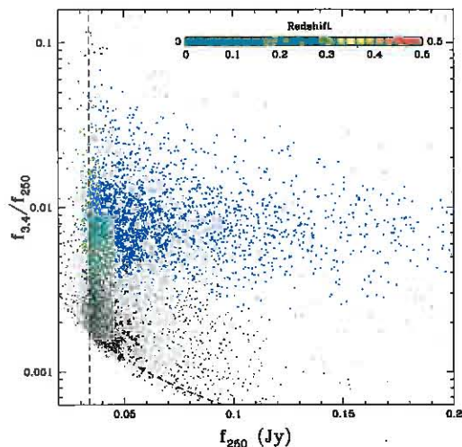
FIG. 2.— Distribution of the 3.4\text{-}250\ \mu\text{m} flux density ratio as a function of 250\ \mu\text{m} flux density for H-ATLAS sources with WISE 3.4\ \mu\text{m} IDs. Colored points have spectroscopic redshifts from the GAMA survey and sources without measured redshifts are indicated by black points. Dashed lines indicate the approximate limits of the H-ATLAS and WISE surveys. The majority of sources with spectroscopic redshifts ( z \lesssim 19.4 ) are well detected by WISE , while the no-redshift sources have small flux density ratios that are inconsistent with “normal” low-redshift galaxies.
