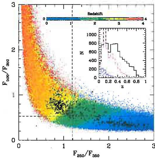
FIG. 3. — FIR flux density ratio for H-ATLAS sources with WISE identifications. Colored grid cells indicate the median redshift of a set of modified blackbody models with temperatures uniformly distributed between 10 and 60 K and emissivity parameters between 0 and 2. Black points indicate sources with 5\sigma detections in all three SPIRE bands, where open squares have spectroscopic redshifts, z < 0.2 , and solid triangles have no spectroscopic or photometric redshift measurement. Dashed lines indicate the median flux density ratios of a stack of sources lacking redshifts. The majority of the no-redshift sources appear to be at z \sim 2 . Inset: Combined distribution of spectroscopic and photometric redshifts for H-ATLAS sources with detections at 3.4\ \mu\text{m} (solid histogram), 12\ \mu\text{m} (dashed), and 22\ \mu\text{m} (hatched). There are 73 sources at z > 1 not shown.
