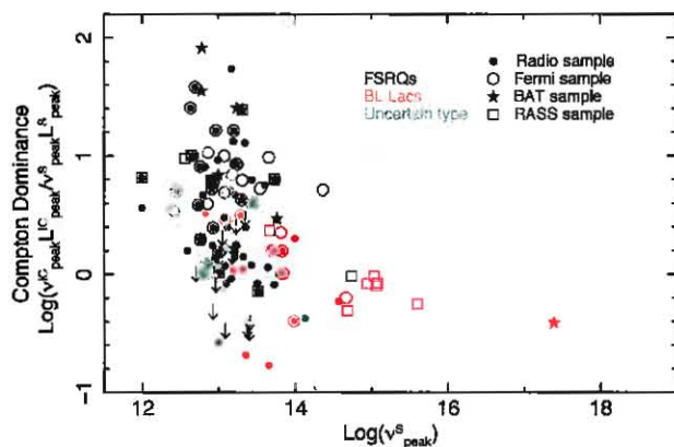
Fig. 21. The logarithm of the Compton dominance is plotted as a function of \log(v^S_{\text{peak}}) for all sources for which v^S_{\text{peak}} and v^{\text{IC}}_{\text{peak}} could be reliably determined.
