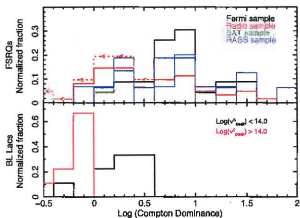
Fig. 22. Distributions of the Compton dominance for FSRQs and BL Lacs of the LSP and HSP type. A significant fraction of FSRQs in the radio, RASS, and BAT samples have not been detected in the \gamma -ray band and therefore only limits to the Compton dominance (shown as a dashed histogram; only the radio sample to avoid confusion) can be calculated. The large difference between the CD distribution of FSRQs in the Fermi -LAT and the other samples illustrates the strong bias that \gamma -ray selection induces.
