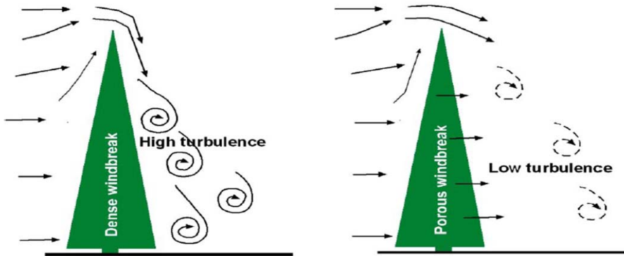
Figure 6. Diagram showing the turbulence caused by windbreaks that are too dense.
