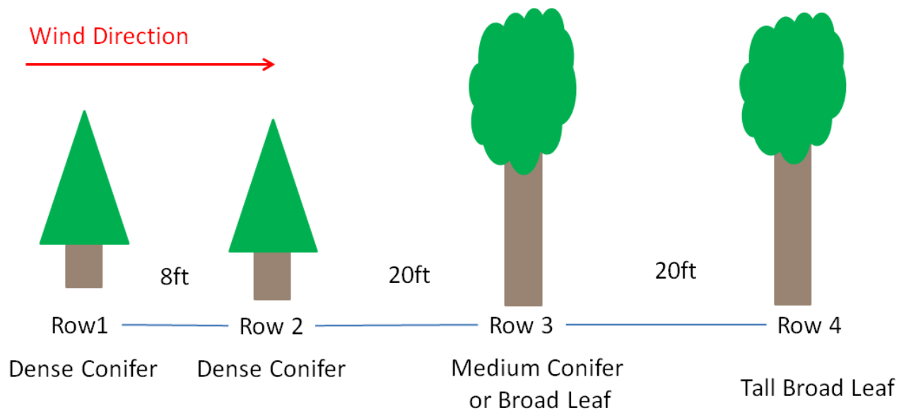
Figure 12. Langley Windbreak Potential 4-row Design.
