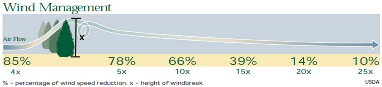
Figure 5. Wind management schematic that shows the relationship between wind speed reduction and height of windbreak. [5]
