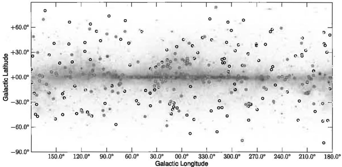
Fig. 24.— All-sky map for energies >1\text{GeV} indicating the positions of the 1FGL sources that are not in the 2FGL catalog (green circles). The red crosses indicate the sources having the flag ‘NC’ in Table 8)
