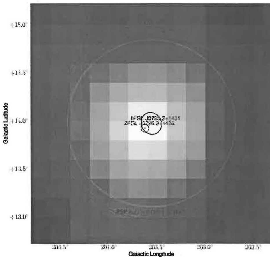
Fig. 25.— A typical example of a 1FGL source associated with a 2FGL source using d_{99.9} . The E > 1 GeV counts map (1 pixel = 0^{\circ}.2 ) was smoothed using a gaussian kernel ( \sigma = 3 pixels). The ellipses represent the 99.9% confidence error regions.
