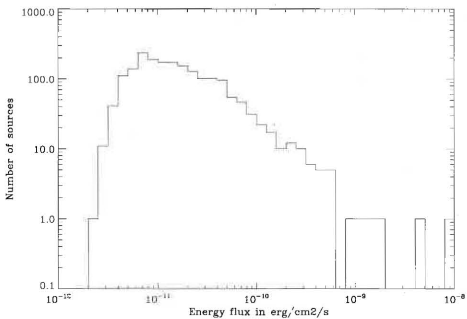
Fig. 7.— Distribution of all sources in 2FGL with respect to \log(\text{Energy flux}) . The low flux threshold is quite sharp around 5 \times 10^{-12} erg cm -2 s -1 , indicating that the TS cut that is applied is not too far from a cut on the energy flux S_{25} over the full band (100 MeV to 100 GeV).
