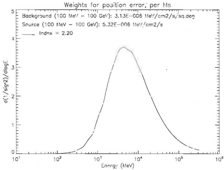
Fig. 33.— Theoretical contribution ( W_l(E) of Eq. A3) to \Delta\theta_0^{-2} per Ms and per \log(E) interval as a function of energy for a TS = 100 power-law source over the average background at |b| > 10^\circ . The assumed photon spectral index is 2.2.
