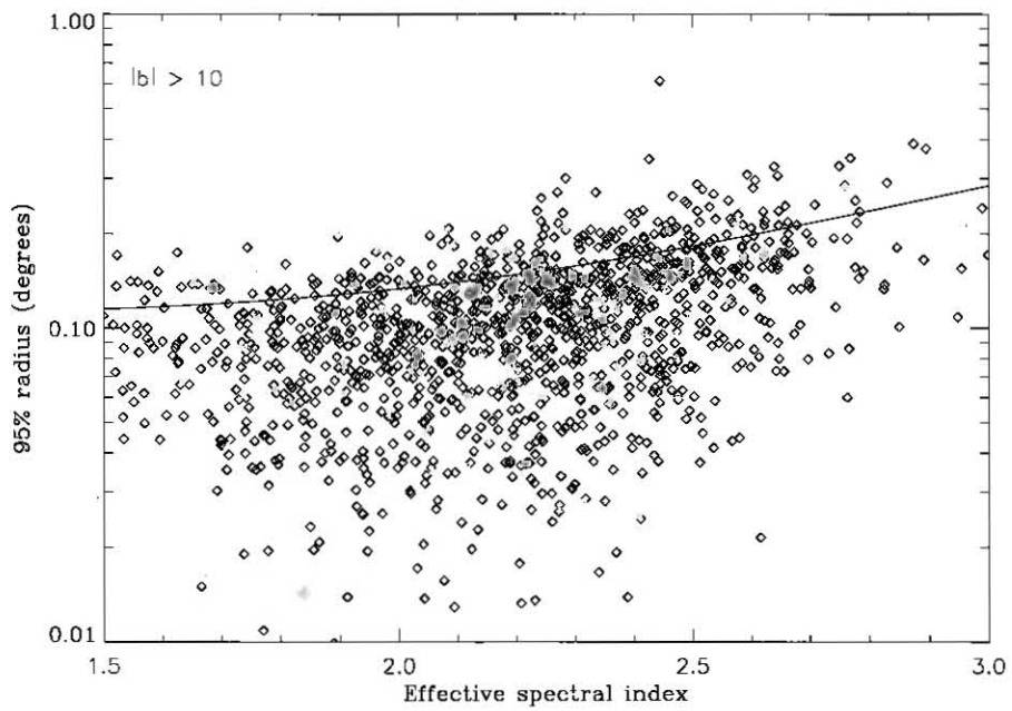
Fig. 34.— 95% error radius of sources at |b| > 10^\circ as a function of spectral index. The line shows the theoretical error radius for an isolated source at the detection threshold of TS = 25 over the average extragalactic background.
