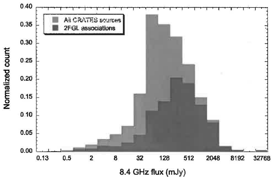
Fig. 30.— Normalized histograms of the 8.4 GHz radio flux of CRATES sources (red: all sources, blue: objects associated with 2FGL sources).
