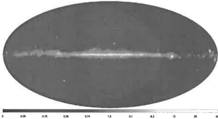
Fig. 1.— Sky map of the energy flux derived from the LAT data for the time range analyzed in this paper, Aitoff projection in Galactic coordinates. The image shows \gamma -ray energy flux for energies between 100 MeV and 10 GeV, in units of 10^{-7} \text{ erg cm}^{-2} \text{ s}^{-1} \text{ sr}^{-1} .
