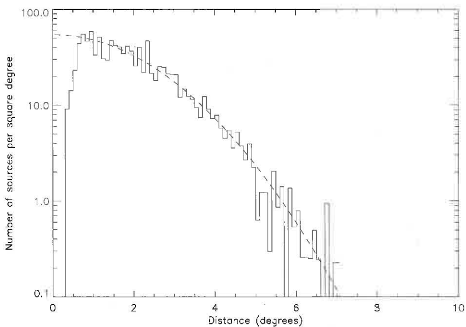
Fig. 14.— Distribution of the distances D_n to the nearest neighbors of all detected sources at |b| > 10^\circ . The number of entries is divided by 2\pi D_n \Delta D_n in which \Delta D_n is the distance bin, in order to eliminate the 2-dimensional geometry. The overlaid curve is the expected Gaussian distribution for a uniform distribution of sources with no confusion.
