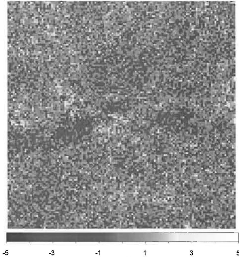
Fig. 35.— Residuals (in \sigma units) in 0.5^\circ pixels over a 60^\circ \times 60^\circ area around the Galactic anticenter, summed over the full energy range (100 MeV to 100 GeV). All sources were fixed to the catalog values and the diffuse parameters were fitted as in an ordinary RoI (§ 3.2). The pixels used in the source fitting process were much smaller. The larger pixels used here allow reducing the statistical fluctuations to 5% in the Galactic plane and 10% at the top and bottom of the plot.
