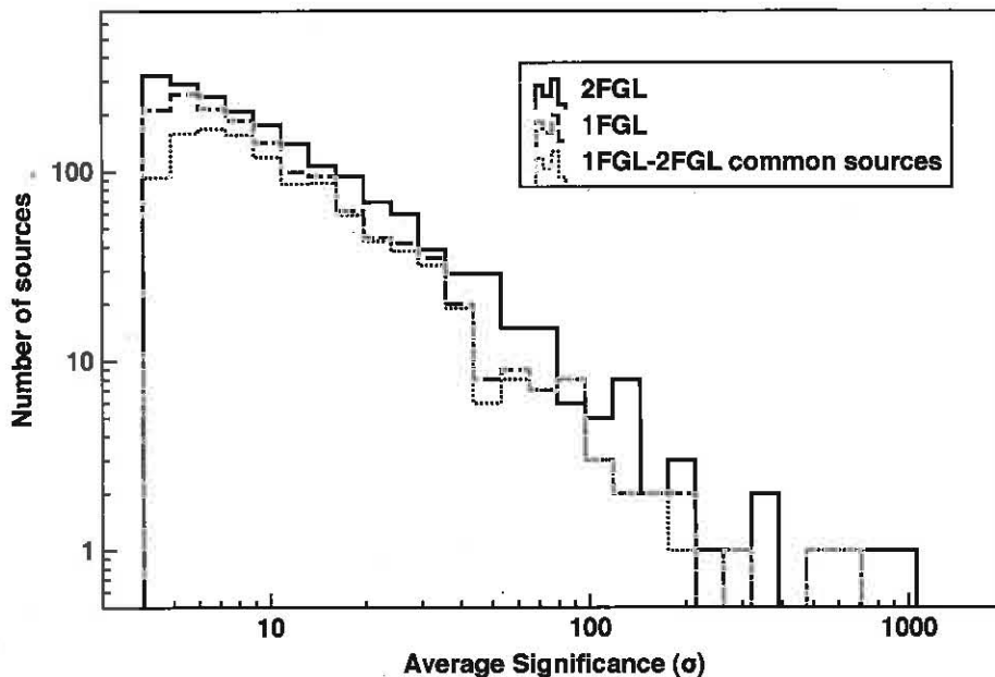
Fig. 23.— Distributions of the significances of the sources in the 1FGL and 2FGL catalogs and of the sources in common between the catalogs. The distribution of the significance for the 1FGL-2FGL common sources is based on the values reported in the 1FGL catalog.
