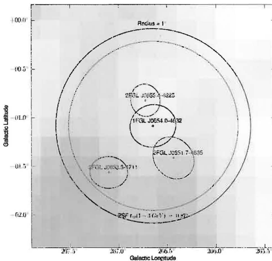
Fig. 27.— A typical example of a 1FGL source that was split in two 2FGL sources. The E > 1 GeV counts map (1 pixel = 0^{\circ}.2 ) was smoothed using a gaussian kernel ( \sigma = 3 pixels). The ellipses represent the 99.9% confidence error regions.
