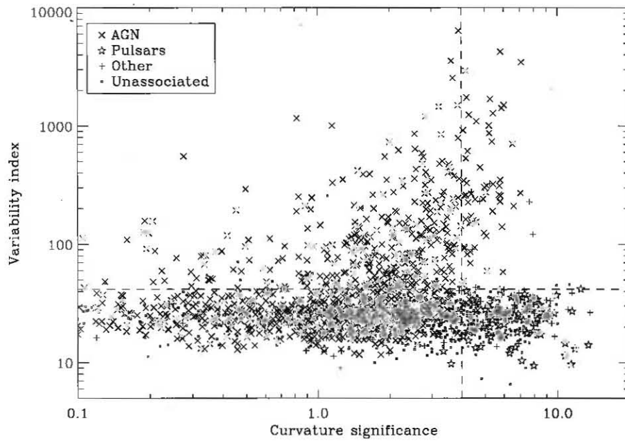
Fig. 19.— Variability index ( TS_{var} in § 3.6) plotted as a function of the curvature significance ( Signif\_Curve in § 3.5) for different broad classes of sources. “AGN” here means any class starting with “ag” or “bz” in Table 6. The horizontal dashed line is set to 41.6, above which sources are likely variable. The vertical dashed line is set to 4.0, above which curved spectra are used.
