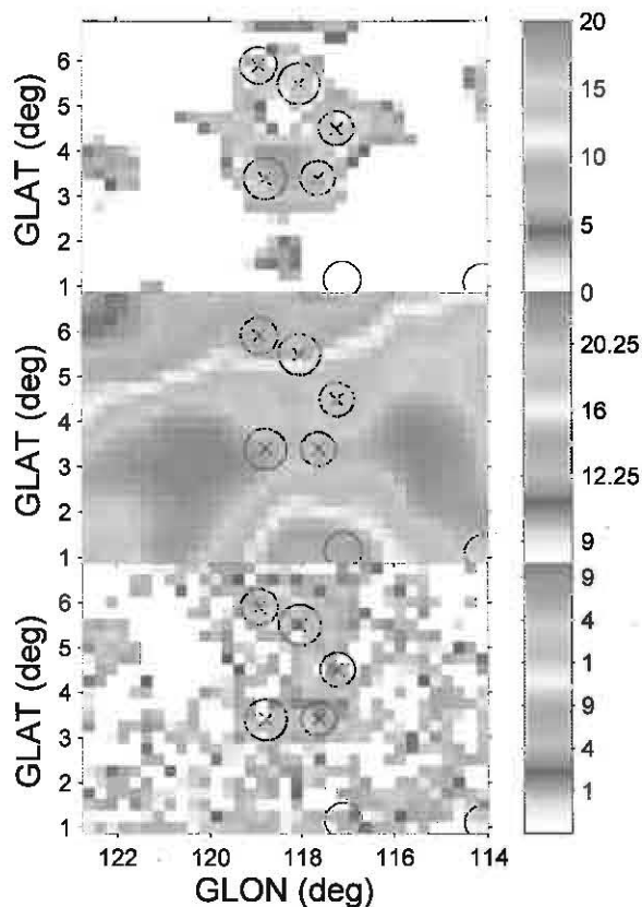
Fig. 16.— From top to bottom: the absolute value of the dust negative residual photon counts incorporated in the diffuse model, the total interstellar photon counts, and the photon residual counts above the diffuse model, all in the 1–11 GeV energy band. The circles mark the effective 50% containment radii of the 2FGL sources for the 1–10 GeV band. The ‘c’ sources are crossed. The photon residual map has been smoothed for display with a \sigma = 0.125 Gaussian. The 2FGL ‘c’ sources are distributed along the rim of a large H II region where the dust temperature correction led to an overestimate of the dust column densities in the ionized gas. The negative dust residuals have artificially reduced the diffuse \gamma -ray intensity in these directions.
