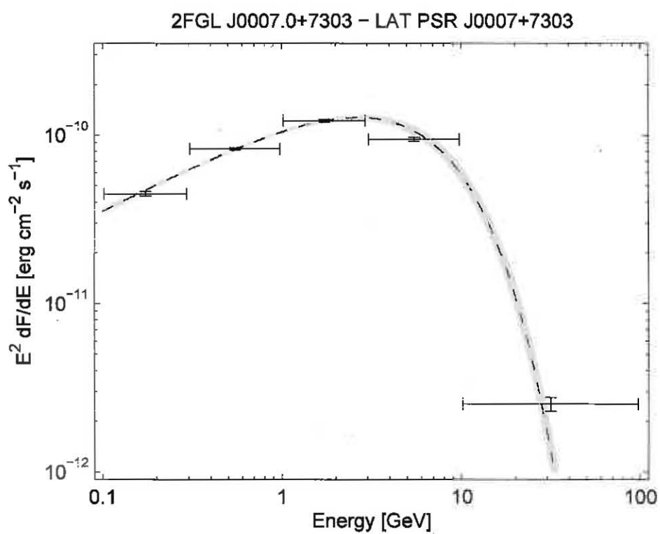
Fig. 9.— Spectrum of the pulsar in CTA1, as an example of an exponentially cutoff spectrum. See Figure 8 for details.
