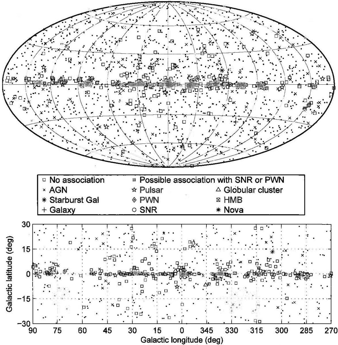
Fig. 17.— Full sky map (top) and blow-up of the inner Galactic region (bottom) showing flagged sources by source class. Sources potentially confused with diffuse emission, i.e., those with a ‘c’ designator in their names (and for which Flag 6 is set) are shown in red; those with any other flag set are shown in blue. Sources with no flag set are shown as small dots.
