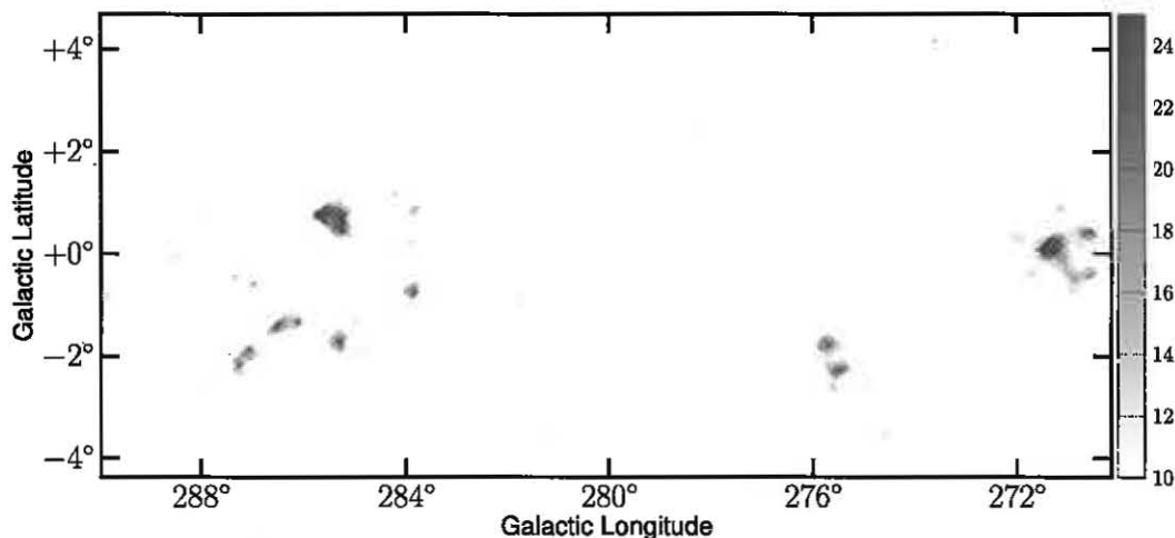
Fig. 4.— A representative map of the TS residuals along the Galactic ridge, corresponding to the final iteration. There are several clusters that could have generated seeds, but did not appear to be isolated point sources under visual inspection.
