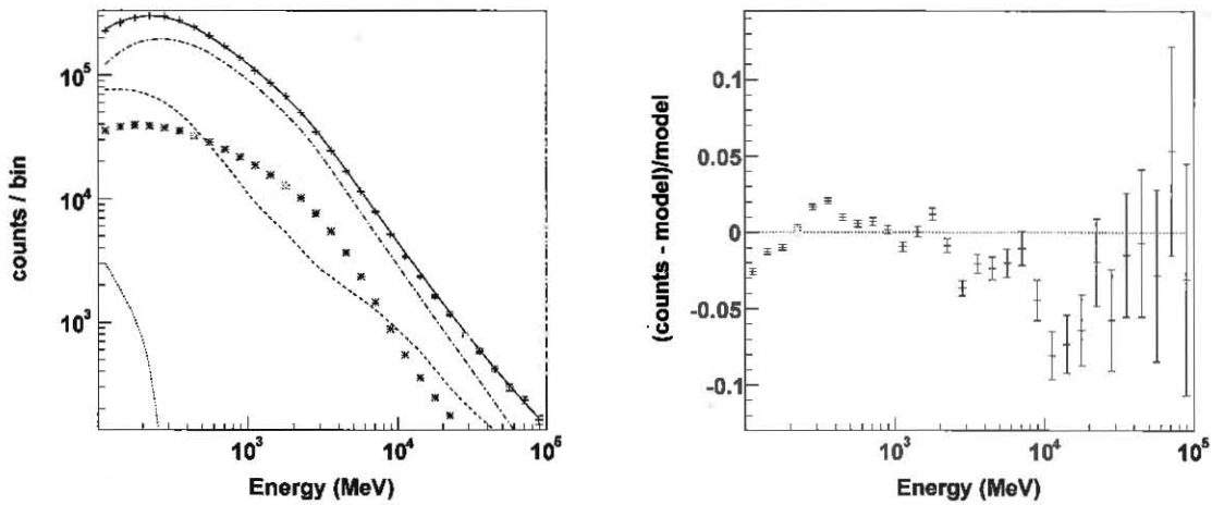
Fig. 36.— Left: Fit to the full spectrum integrated over the same anticenter region as in Figure 35. The spectral bins are the same as in the source fitting process. The dotted, dashed and dash-dotted lines are the Earth limb, isotropic and Galactic components, respectively. The asterisks show the total source contribution (dominated by the Geminga and Crab pulsars). The full line is the sum of all model contributions, to be compared with the data (plus signs). The statistical errors on the data are shown but barely visible except at high energy. Right: Fractional residuals (data/model-1) with statistical error bars. The residuals are statistically significant because of the very large number of events ( 2.8 \times 10^6 over that area) but are only a few percent.
