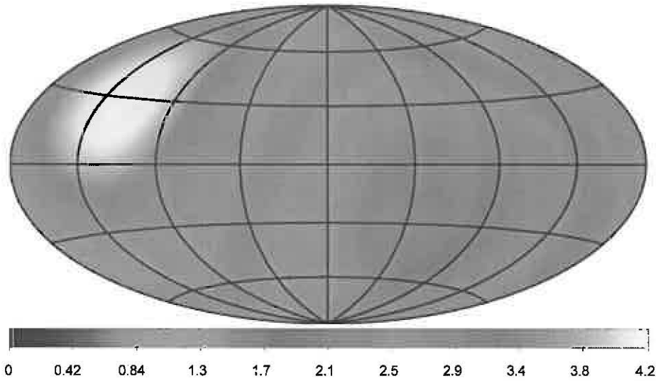
Fig. 2.— Exposure of the LAT for the period September 2009 to July 2010 when the rocking angle was 50^\circ , Aitoff projection in Galactic coordinates. The units are equivalent on-axis exposure at 1 GeV in Ms.
