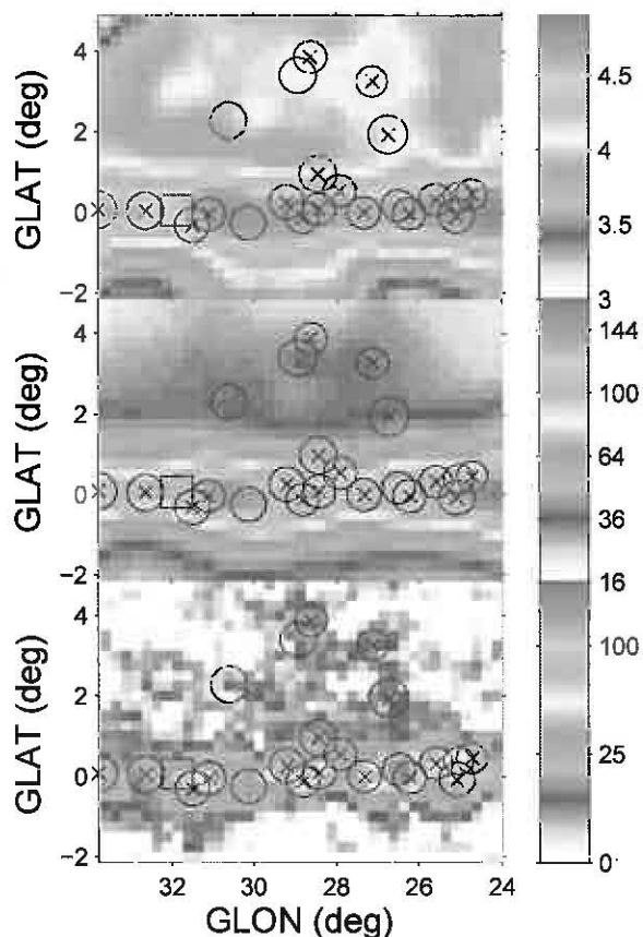
Fig. 15.— From top to bottom: the CO contribution to the interstellar photon counts, the total interstellar photon counts, and the photon residual counts above the model for diffuse \gamma -ray emission, all in the 1–11 GeV energy band. The circles mark the effective 50% containment radii of the 2FGL sources for the 1–10 GeV band. The ‘c’ sources are crossed. The square notes an identified source. The photon residual map has been smoothed for display with a \sigma = 0^{\circ}.125 Gaussian. The 2FGLc sources seen above the Galactic plane, with TS ranging from 26 to 75, follow an extended and clumpy excess of interstellar emission
