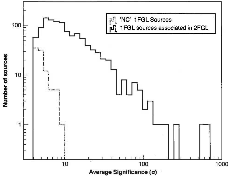
Fig. 29.— Distribution of the significances of the unconfirmed 1FGL sources and of the 1FGL sources associated with sources in the 2FGL catalog.
