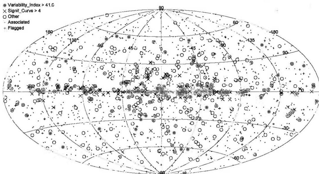
Fig. 31.— Sky distribution of associated (dots) and unassociated sources (large symbols). Sources that were flagged are marked by a plus. In particular, we mark variable unassociated sources ( TS_{var} > 41.6 ) using filled blue circles, unassociated sources with a curved spectrum ( Signif\_Curve > 4 ) by red crosses, and all other unassociated sources by open black circles.
