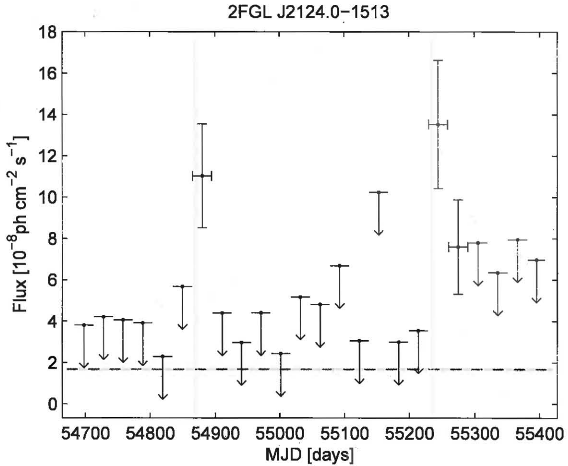
Fig. 13.— Light curve for the unassociated source 2FGL J2124.0-1513 (100 MeV to 100 GeV). Time periods in which the sun is closer than 2.5^\circ to the source are marked with yellow vertical bands. In this case, a large fraction of the detection significance is accumulated during these periods, and the source is flagged as suspicious in the catalog.
