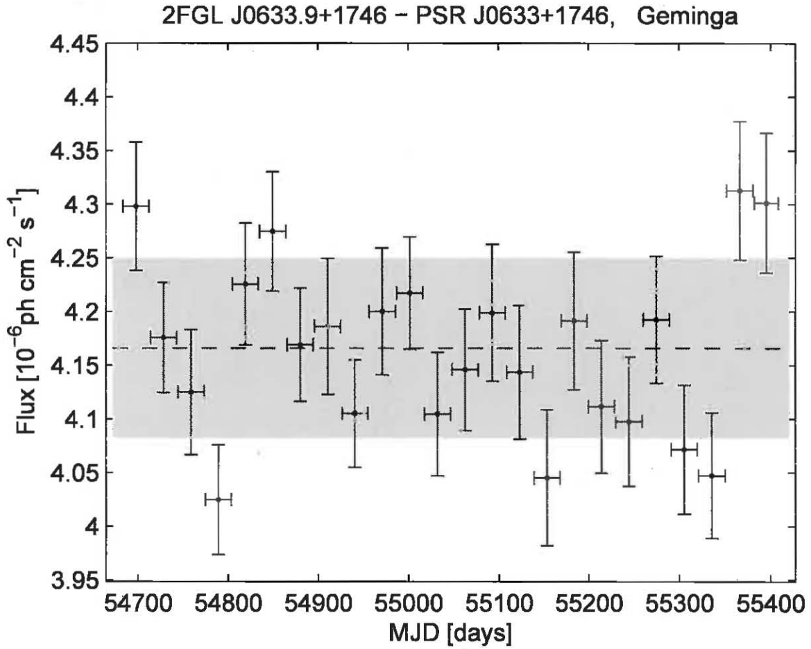
Fig. 12.— Light curve for the bright pulsar Geminga (100 MeV to 100 GeV). The gray band depicts the size of the 2% systematic correction applied to the calculation of the variability index. The error bars on the flux points show the statistical errors only.
