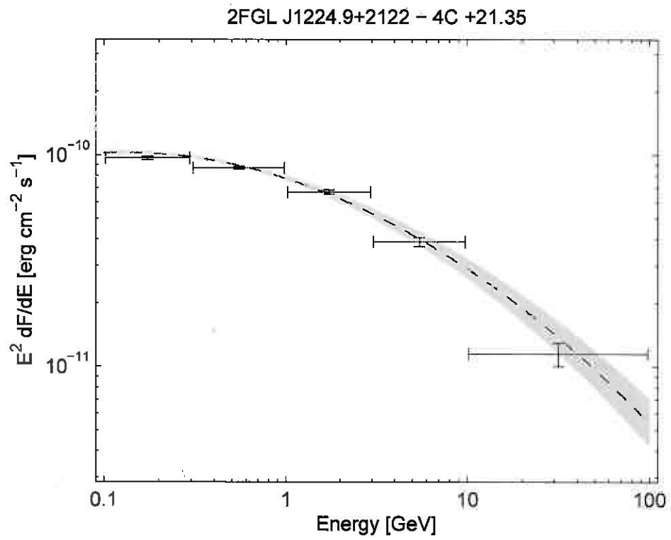
Fig. 10.— Spectrum of the bright AGN 4C +21.35, as an example of a LogParabola spectrum. See Figure 8 for details.
