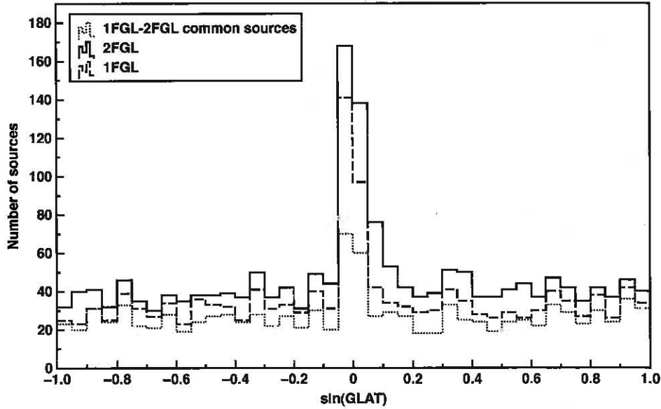
Fig. 20.— Distributions of the Galactic latitude of the 1FGL and 2FGL sources and of the sources in common between the 1FGL and 2FGL catalogs.
