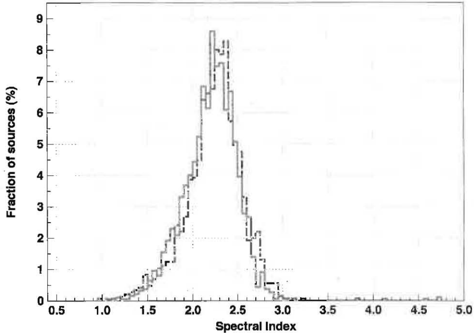
Fig. 21.— Distributions of the spectral index for the 1FGL (1451 sources, dashed line) and for the 2FGL (1873 sources, solid line) catalogs.
