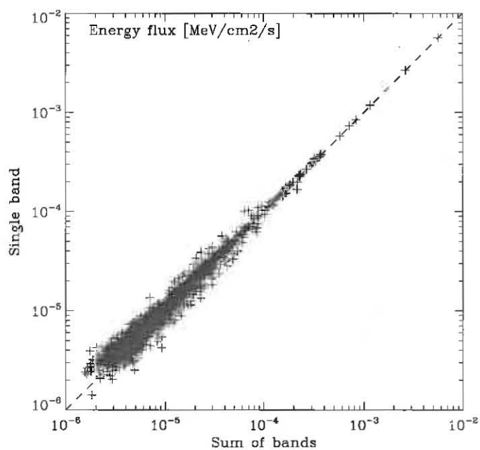
Fig. 5.— Comparison of estimates of the energy flux from 100 MeV to 100 GeV S_{25} from the sum of bands (abscissa) and the fit to the full band (ordinate). No obvious bias can be observed.
