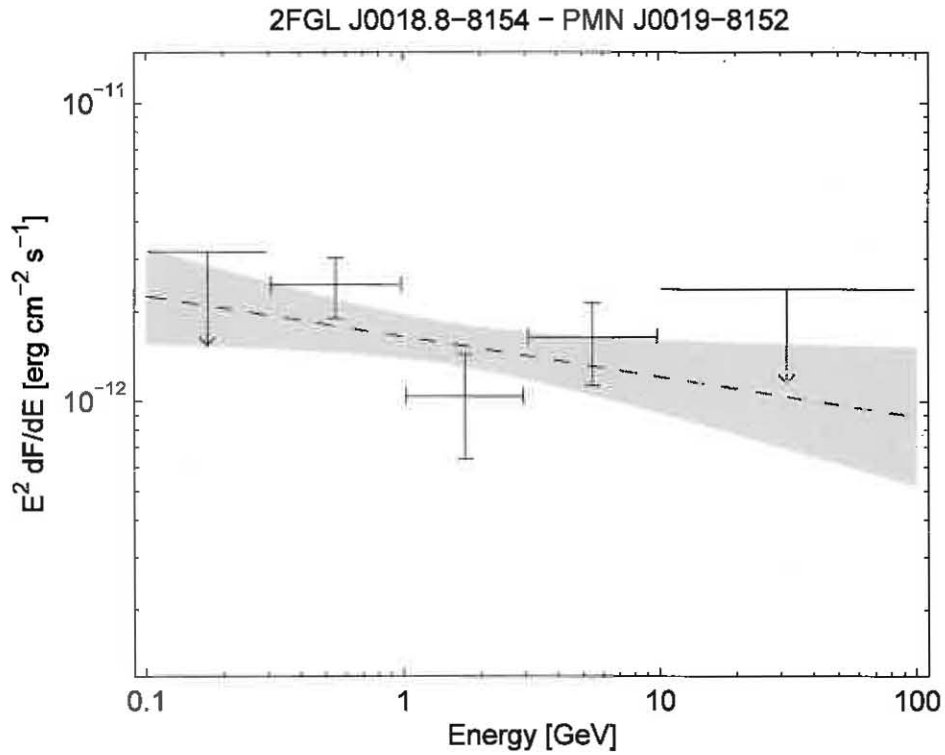
Fig. 8.— Spectrum of a faint AGN, as an example of a power-law spectrum. The fit over the full band (dashed line) is overlaid over the five band fluxes converted to \nu F_\nu units. The grey shaded area (butterfly) shows the formal 1 \sigma statistical error on \log(\text{differential flux}) as a function of energy, obtained using the covariance matrix involving the parameters of that particular source. The upper limits (here the lowest-energy and highest-energy bands) are 2 \sigma .
