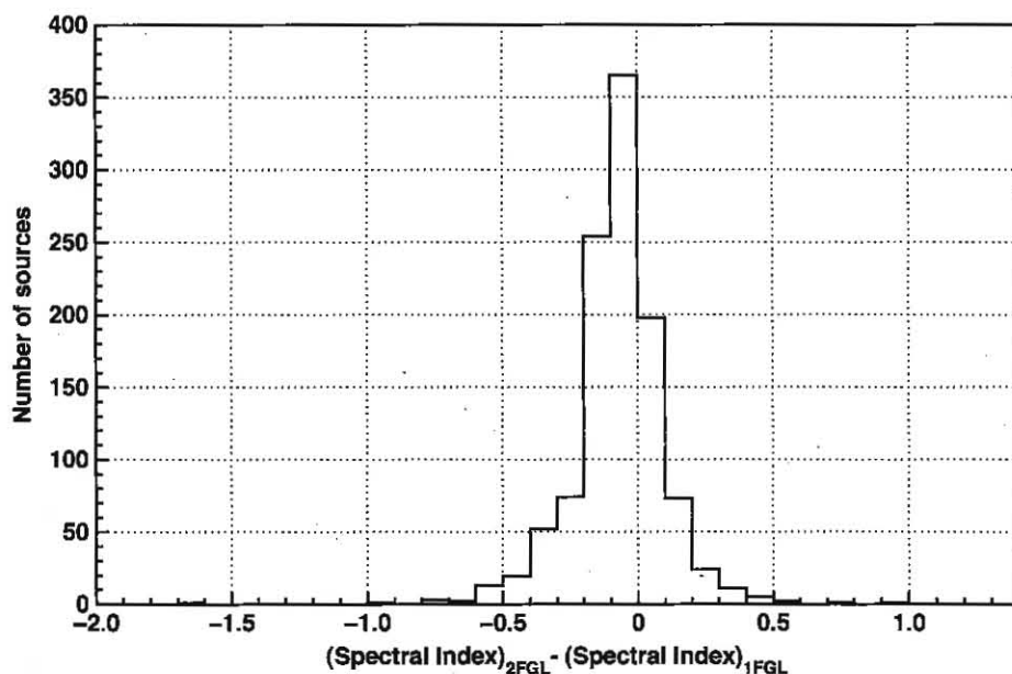
Fig. 22.— Distribution of the difference \Gamma_{2FGL} - \Gamma_{1FGL} for the 1099 sources in common between the 1FGL and 2FGL catalogs.
