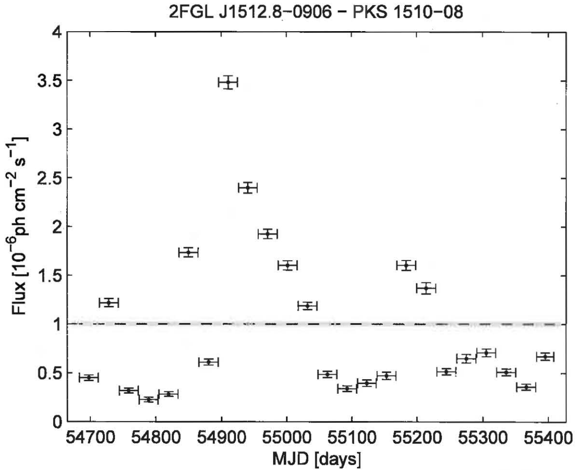
Fig. 11.— Light curve for the bright blazar PKS 1510-089 in the full energy range (100 MeV to 100 GeV). The dashed line depicts the average flux from the analysis of the full 24-month dataset.
