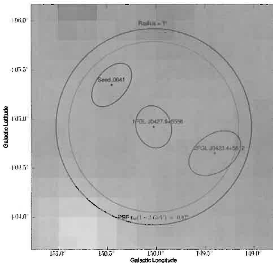
Fig. 26.— A typical example of a 1FGL and a 2FGL source having an angular separation greater than d_{99.9} but less than 1^\circ . In this particular case there is also a seed (candidate source considered in the 2FGL analysis) separated by less than 1^\circ from the 1FGL source. The E > 1 GeV counts map (1 pixel = 0.2^\circ ) was smoothed using a gaussian kernel ( \sigma = 3 pixels). The ellipses represent the 99.9% confidence error regions.
