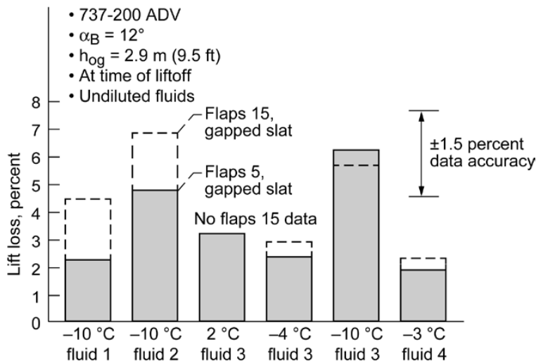
Figure 2.—Summary of fluid effects on lift coefficient from B737-200ADV flight test trials, from Hill and Zierter (Ref. 13).
