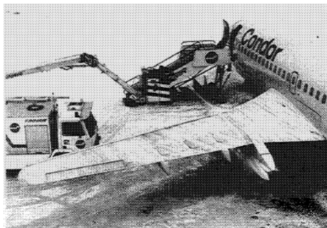
Figure 1.—Application of anti-icing fluid to B737-200ADV during flight test trials at Kuopio, Finland, in 1988, from Hill and Zierten (Ref. 13). Reprinted with permission of the American Institute of Aeronautics and Astronautics.
