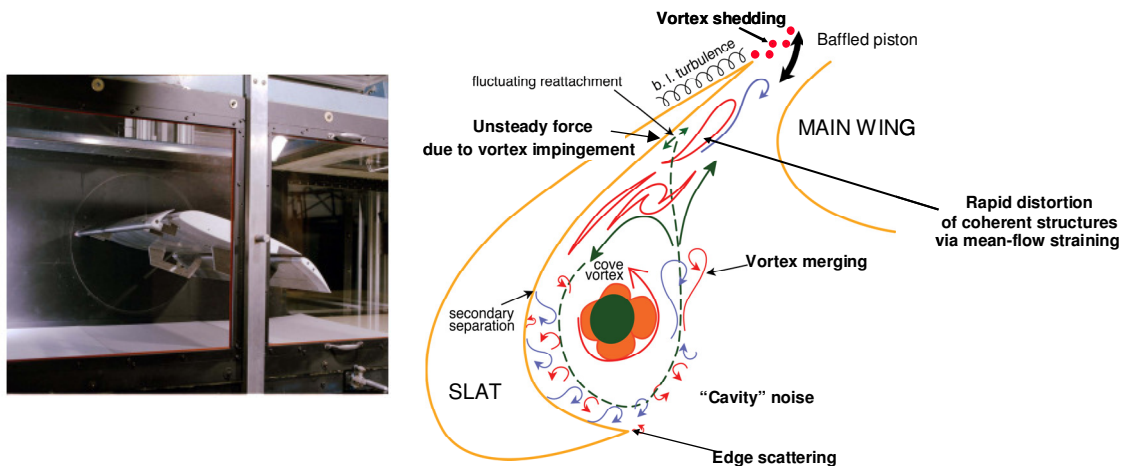
(a) 30P30N airfoil installed in the Basic Aerodynamics Research Tunnel (b) Potential sources and physical mechanisms behind noise generation near a leading edge slat Fig. 2 Category 7 of BANC-II Workshop: 30P30N 3-Element, Simplified High-Lift Configuration
