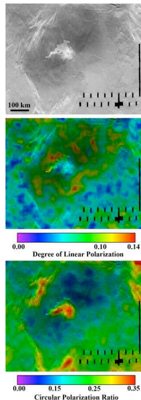
Figure 1: Radar polarimetry from the Arecibo Observatory radar system (2380 MHz) demonstrates that a radar-dark region surrounding the crater Galina on Venus is covered in fine-grained mantling material [2]. From the Magellan data (top), it is not clear whether the dark region has been swept clear of rocks or whether it is mantled. Increased DLP values (middle) reveal that the radar wave penetrates into a surficial deposit, while low CPR values (bottom) demonstrate that the deposit is rock-poor. This dark area is therefore a smooth deposit of cm-sized or smaller material generated by the impact.
