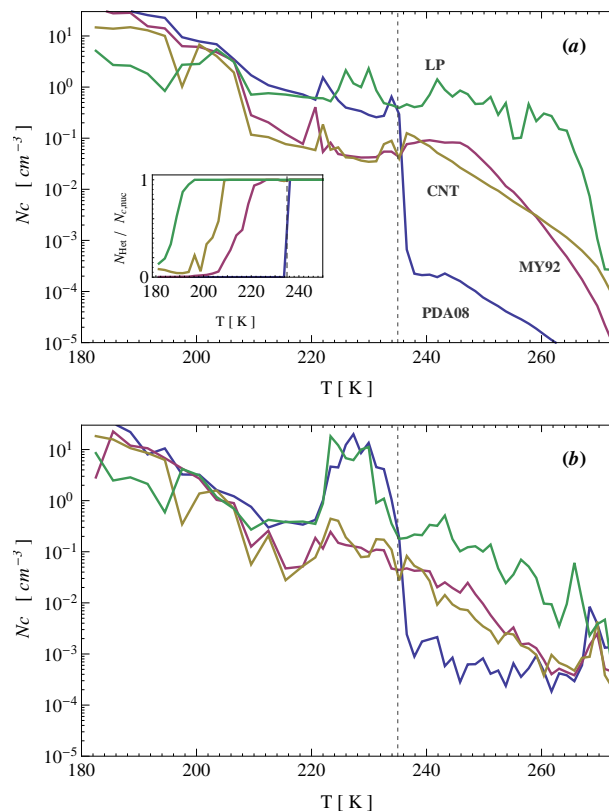
Fig. 4. (a) Average number of nucleated ice crystals, N_{c, \text{nucl}} as a function of temperature for the simulations considered in this study. The inset is the fraction of crystals nucleated heterogeneously, N_{\text{het}}/N_{c, \text{nucl}} . (b) Average number concentration of ice crystals N_c as a function of temperature. The vertical dashed line marks the homogeneous freezing temperature threshold.
