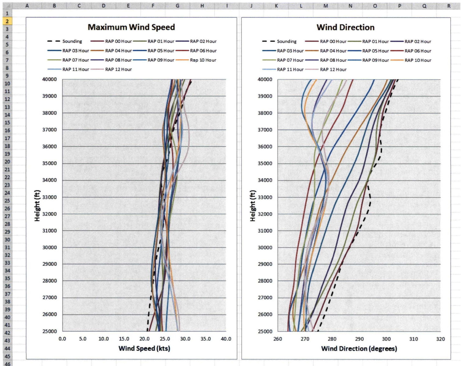
Figure 3. Screen shot of the RAP tab in GUI showing the observed (dashed black line) and model forecast (solid lines) profiles of wind speed (left) and direction (right).
