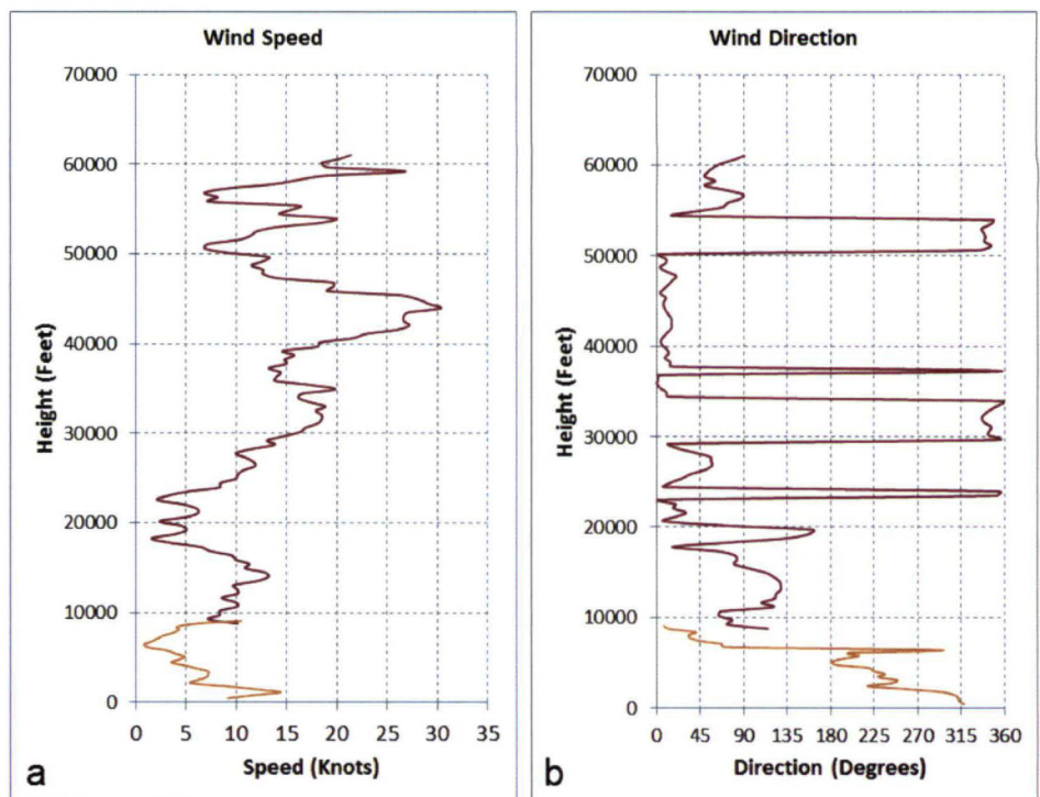
Figure 5. Wind speed (a) and wind direction (b) profiles from the 1201 UTC 3 Jul 2012 915 MHz profiler (orange lines) and the 1155 UTC 3 Jul 2012 50 MHz profiler (dark red lines) plotted in Excel.
