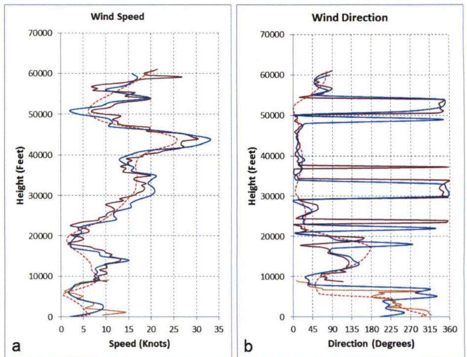
Figure 7. Wind speed (a) and wind direction (b) profiles at the RAP model initial time of 1200 UTC 3 Jul 2012 (dashed red line) overlaid on the observations from AMPS, 50 MHz and 915 MHz profiles as in Figure 3.
