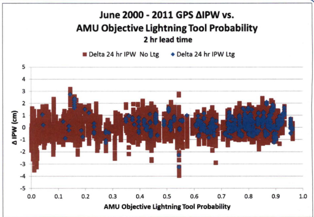
Figure 13. Scatter plot of AMU Objective Lightning Probability tool daily probability vs. \Delta IPW over a 24-hour period and a 2-hour lead time before a CGLSS flash occurred (blue diamond, lightning occurred) and when a CGLSS flash did not occur (red square, lightning did not occur) for the month of June during the entire POR.
