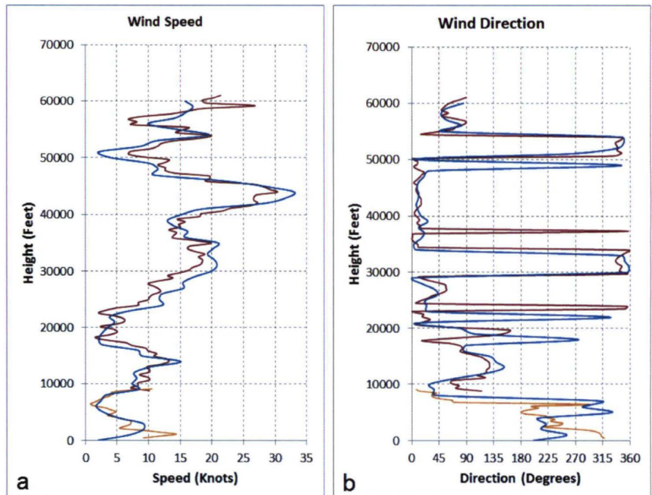
Figure 6. Wind speed (a) and wind direction (b) profiles from 1018 UTC 3 Jul 2012 AMPS (blue lines) and the 50 MHz and 915 MHz profiles as in Figure 5.
