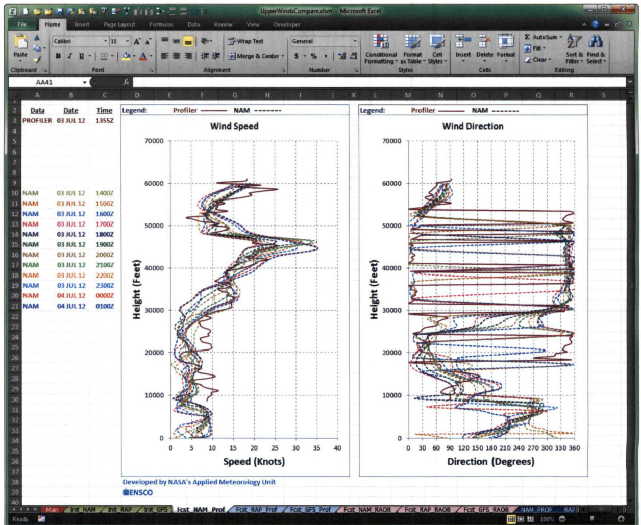
Figure 8. Wind speed (left) and wind direction (right) profiles from the 1355 UTC 3 Jul 2012 50 MHz profiles as in Figure 3 plus the 1400 UTC 3 Jul 2012 - 0100 UTC 4 Jul 2012 NAM model forecasts (dashed lines) plotted in Excel.
