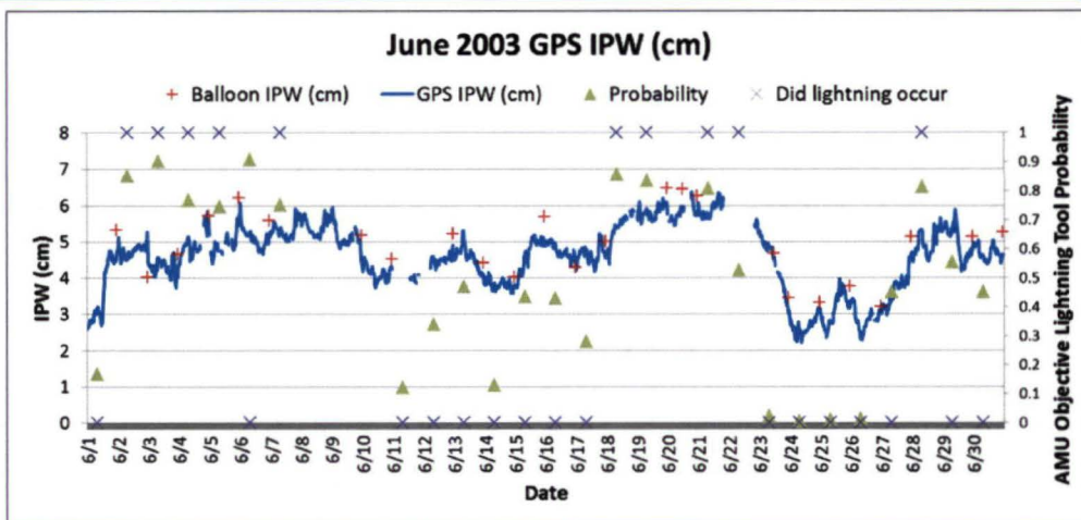
Figure 10. The June 2003 time series of IPW in centimeters (cm) from GPS observations made at the Cape Canaveral, Fla., site (left vertical axis, blue line), integrated precipitable water from the CCAFS soundings (red pluses), the AMU Objective Lightning Probability tool daily output (right vertical axis, green triangles), and lightning occurrence (purple Xs) within the 5 NM KSC/CCAFS lightning warning circles (see Figure 12).
