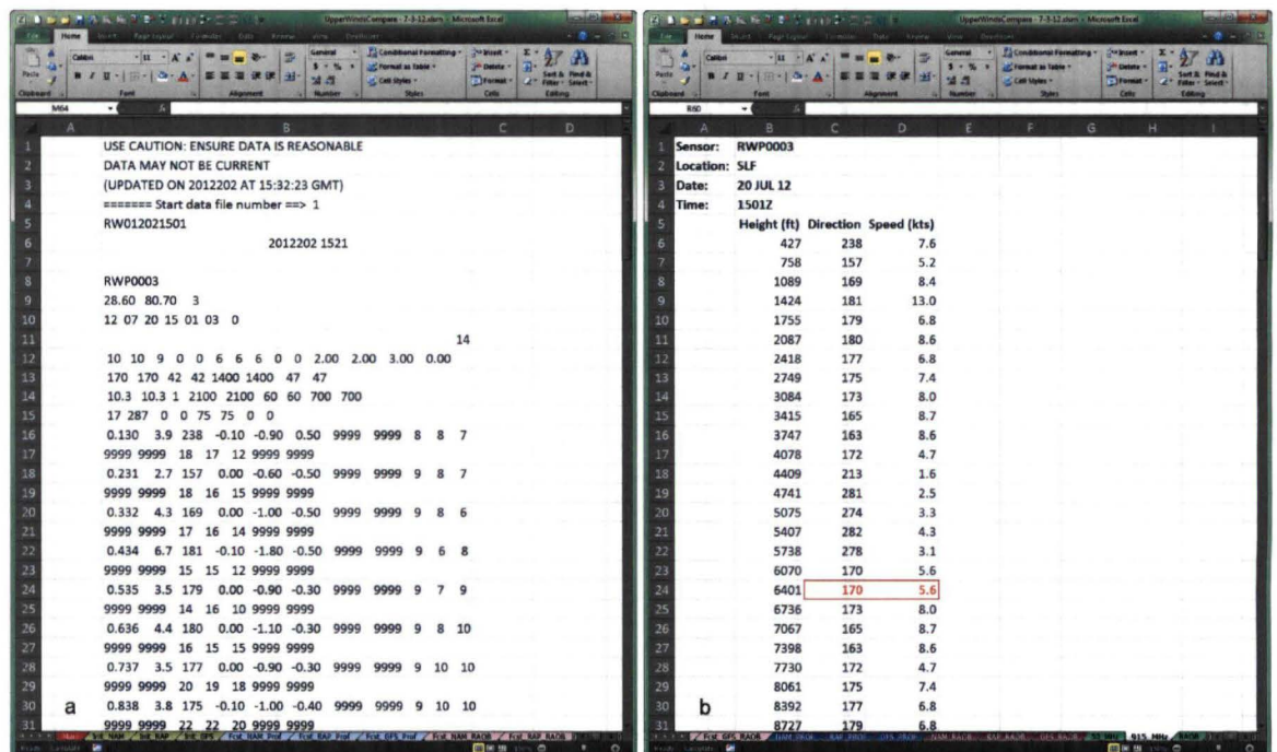
Figure 4. 915 MHz profiler observations (a) after being ingested into Excel and (b) after unneeded parameters were removed and data was quality controlled, displaying the sensor type and location, date, time, height, wind direction and speed. The red text surrounded by the red box in (b) shows that it was copied from the height below (line above) to replace missing data.
