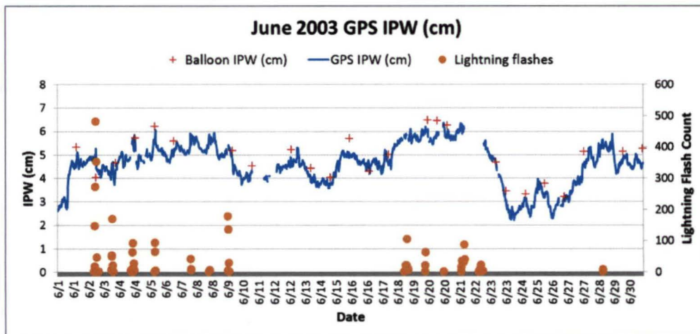
Figure 11. The June 2003 time series of IPW in centimeters (cm) from GPS observations made at the Cape Canaveral, Fla., site (left vertical axis, blue line), integrated precipitable water from the CCAFS soundings (red pluses), and the CGLSS flash count (right vertical axis, orange circles) of lightning that occurred within the 5 NM KSC/CCAFS lightning warning circles (see Figure 12).
