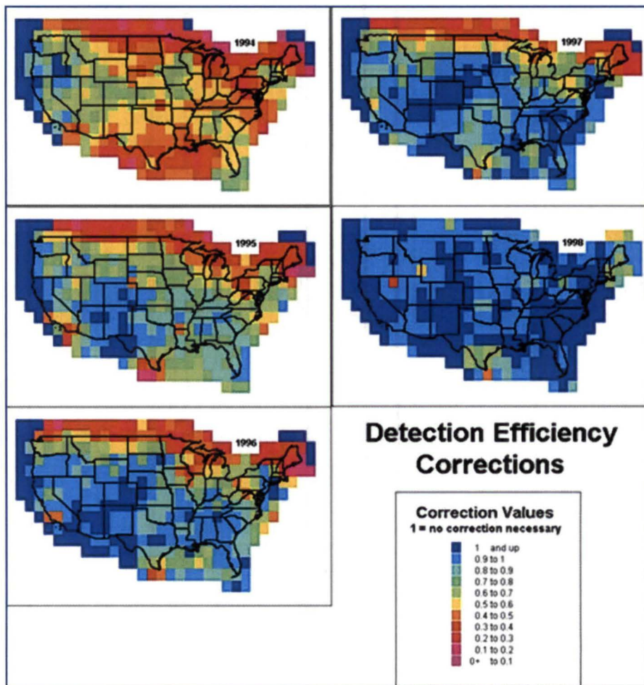
Figure 1. 1994-1998 NLDN DE corrections relative to 1999 values. The grid cell size is 2°x2° latitude/longitude (image created by Vaisala).
