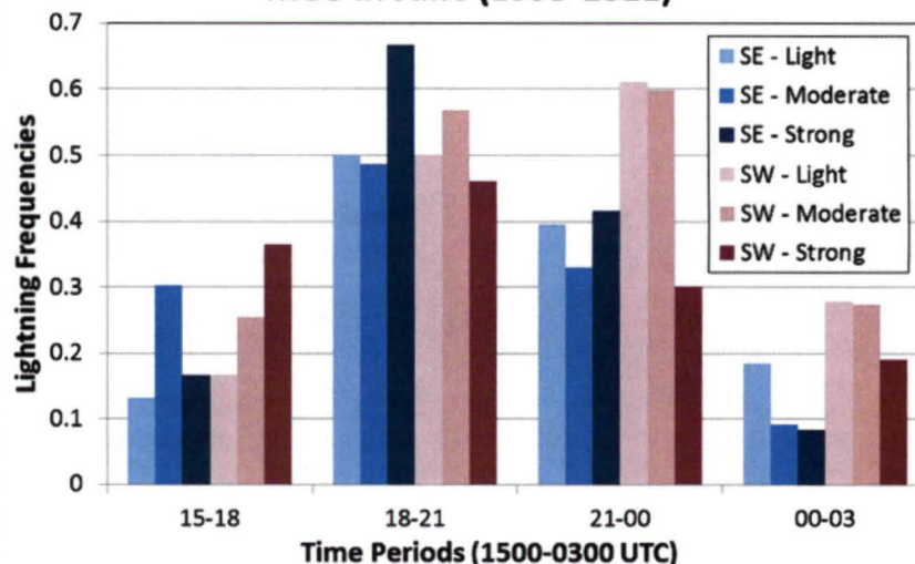
Figure 2. The frequencies of lightning occurrence for the southeast (SE) and southwest (SW) flow regimes for (top) the values of the previous POR and (bottom) the three-category ranges of light, moderate and strong flow.
