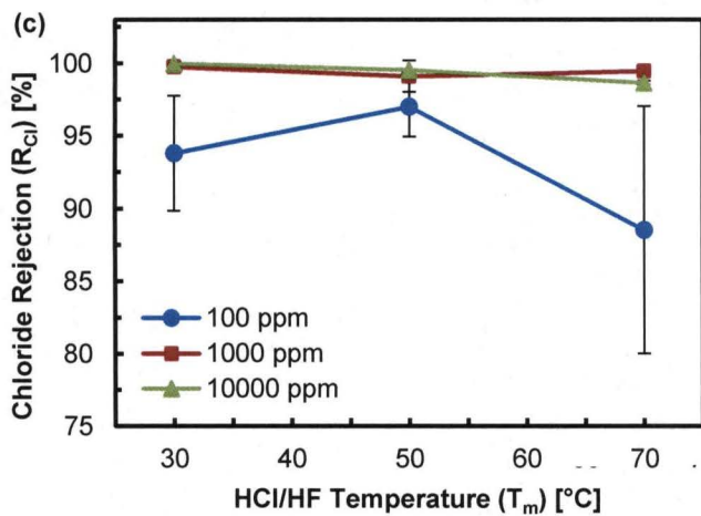
Fig. 4. Chloride rejection by Nafion membranes as a function of HCl/HF solution temperature and concentration, with membranes of thickness 51 mm (a), 127 mm (b), and 254 mm (c).
