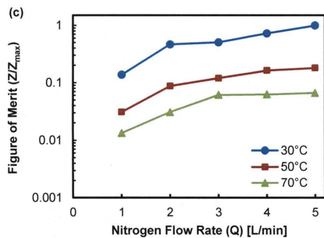
Fig. 10. Normalized figure of merit as a function of gas-side nitrogen flow rate and liquid-side acid solution temperature, with acid solution concentration of 10000 ppm and membrane thicknesses of 51 \mu\text{m} (a), 127 \mu\text{m} (b), and 254 \mu\text{m} (c).
