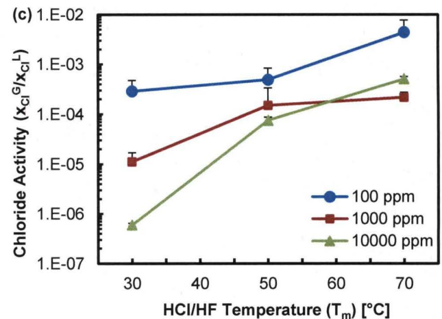
Fig. 5. Ratio of chloride gas-side activity to liquid-side activity as a function of HCl/HF solution temperature and concentration, at membrane thickness of 51 mm (a), 127 mm (b), and 254 mm (c).
