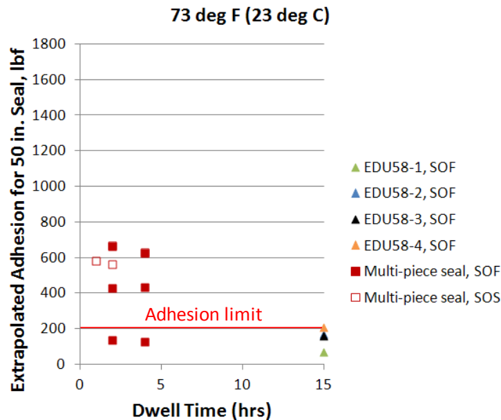
Figure 12.—Extrapolated adhesion loads for 50 in. diameter versions of candidate seal designs based on measured adhesion for untreated subscale seals in the SOF and SOS mating configurations for various dwell times at 73\text{ }^{\circ}\text{F} ( 23\text{ }^{\circ}\text{C} ).
