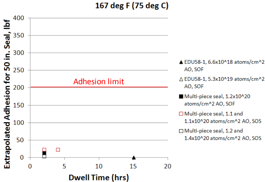
Figure 16.—Extrapolated adhesion loads for 50 in. diameter versions of candidate seal designs based on measured adhesion for AO pretreated subscale seals in the SOF and SOS mating configurations for various dwell times at 167 °F (75 °C).
