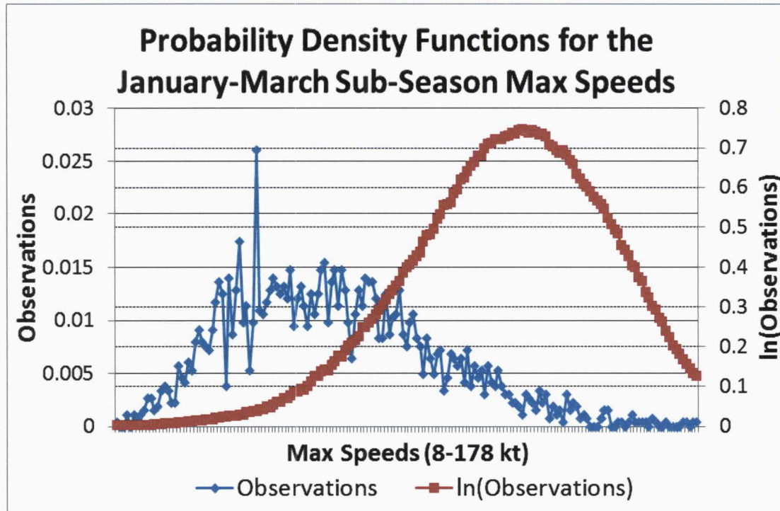
Figure 2. The PDFs of the maximum speed observations (blue, left axis and solid grid lines) and ln of the observations (red, right axis and dotted grid lines).
