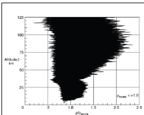
Figure 1. Mars Atmospheric Density Uncertainty, Ref [2].
