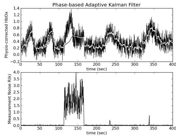
Figure 1 Calculated R (bottom) used to filter the [HbO] trace (top, filter output in negative). The phase variance from a rolling window looking back 1s is used to calculate R . Q was set to 1e-4 .
