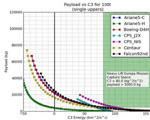
Fig. V.3: Beyond LEO performance of the same stages as V.2 with launch vehicle capability growing from 70 up to 100 metric tons
