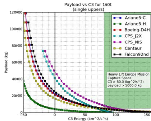
Fig. V.4: Beyond LEO performance of the same stages as V.3 with launch vehicle capability growing from 100 up to 160 metric tons
