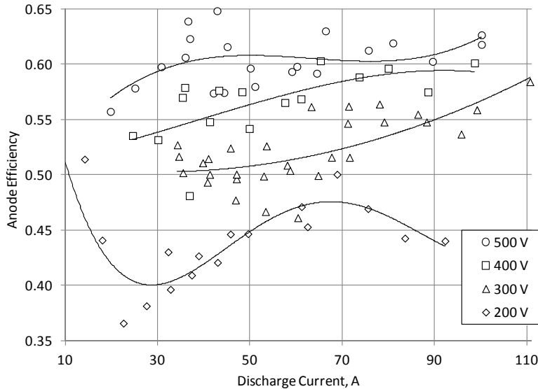
Figure 9.—Anode efficiency as a function of discharge current at various discharge voltages for the laboratory model NASA-457M during operation with high magnetic fields. Data are from References 7 and 8.
