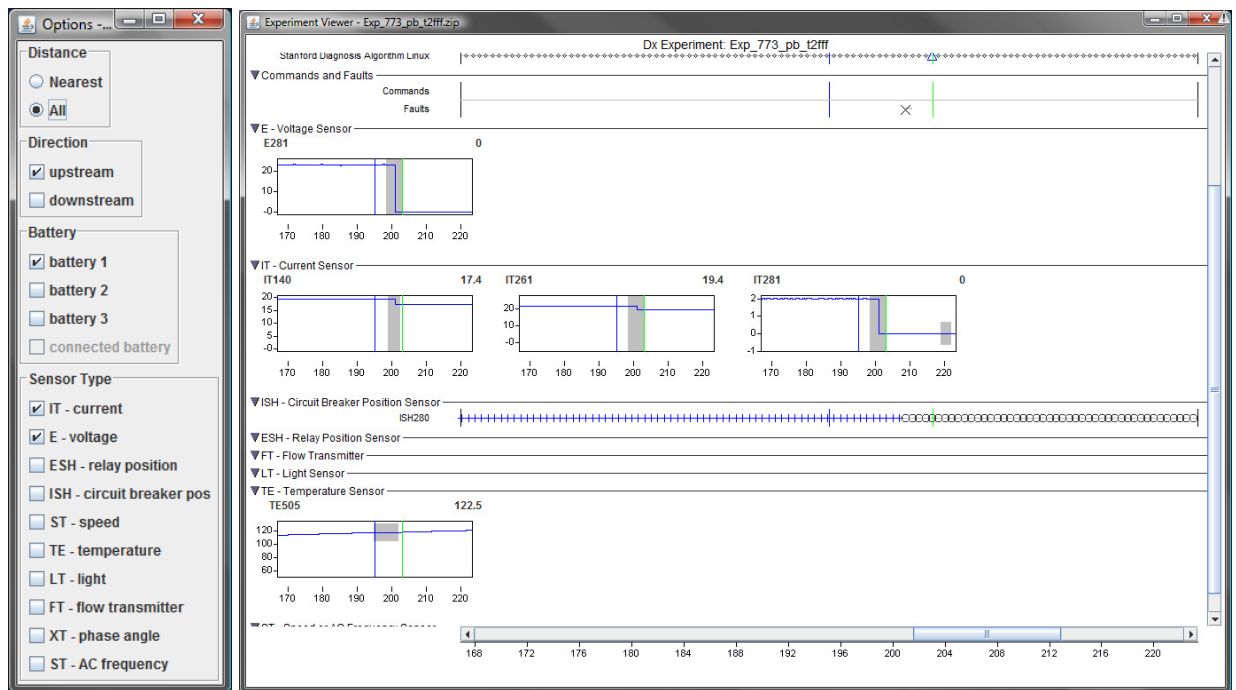
Figure 3. The control panel at left enables users to specify criteria for filtering or highlighting data in the schematic display and in the time-oriented data display. Scrollable timelines and time-series graphs at right help users see temporal data patterns such as coincident sensor data changes.
