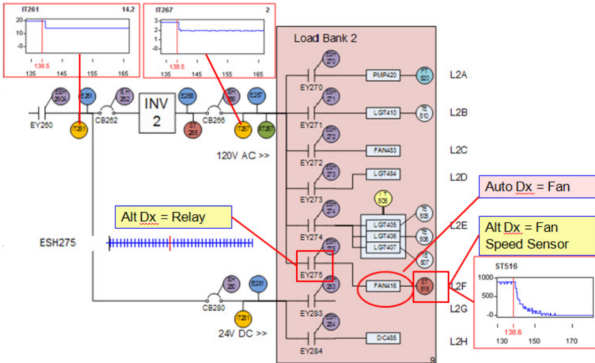
Figure 2. Portion of the ADAPT circuit near fan FAN416, suspected of failing, and graphs of sensor data that are relevant to cross-checking this suspected failure. Rectangles indicate alternate diagnoses.
