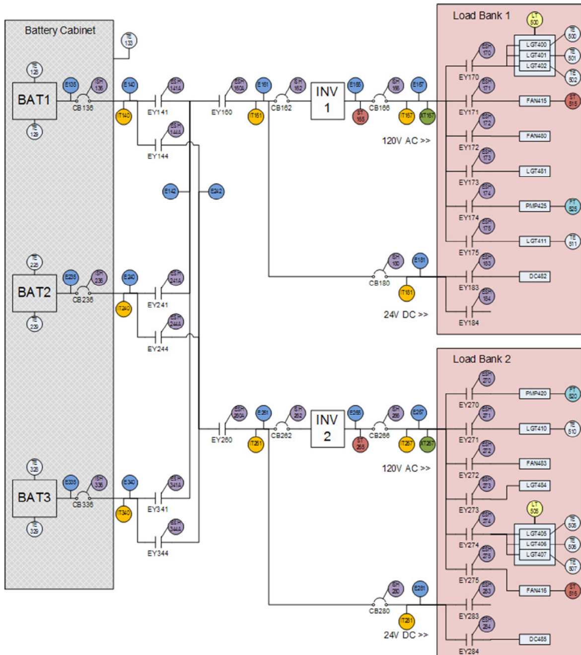
Figure 1. Schematic of the ADAPT electrical system used by the Diagnosis Competition, Tier 2.
