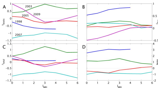
Fig. 5. Global flux anomaly as a function of time-lag for 5 El Niño events from 1997–2009. El Niño events (colored lines) indexed by year (Panel A). Lags ( l_{MEI} ) from 0 to 6 months shown; flux anomaly always lags MEI. Flux anomalies ( \text{Pg C yr}^{-1} ) are Δ biotic (Panel A), Δ fire (Panel B), Δ total (Panel C), and Jena inversion (Panel D). The 1997/1998 event (blue line) cannot be calculated with a lag of 5 or greater as it began in April and a time delay of 5 or more months was not observed. A positive sign indicates increased outgassing of CO 2 to the atmosphere.
