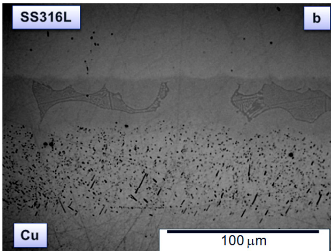
Figure 3.—Optical micrographs of 316L stainless steel brazed to copper with (a) AMDRY 936 and (b) AMDRY 930.
