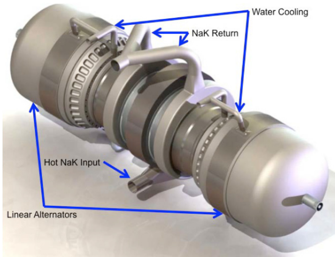
Figure 1.—TDU power conversion unit design (Sunpower, Inc.).
