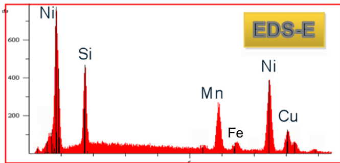
Figure 9.—Platelets formed inside the AMDRY 930 brazed section, near the braze/Cu interface showing similar composition as the one near the SS/braze interface EDS-B of Figure 8.
