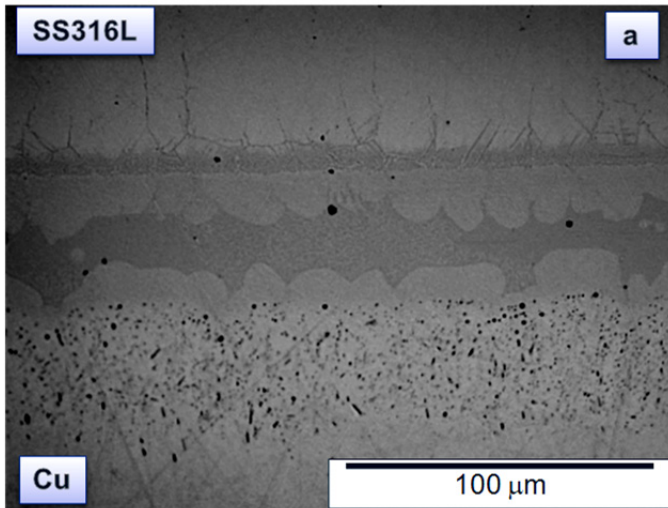
Figure 2.—Group of brazed samples aged at 823 K (550 °C) for 1000 hr in vacuum.
