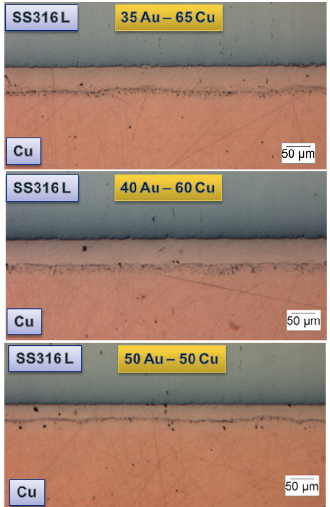
Figure 10.—Optical micrographs of stainless steel brazed to copper using gold-copper braze alloys showing relatively good bonding.
