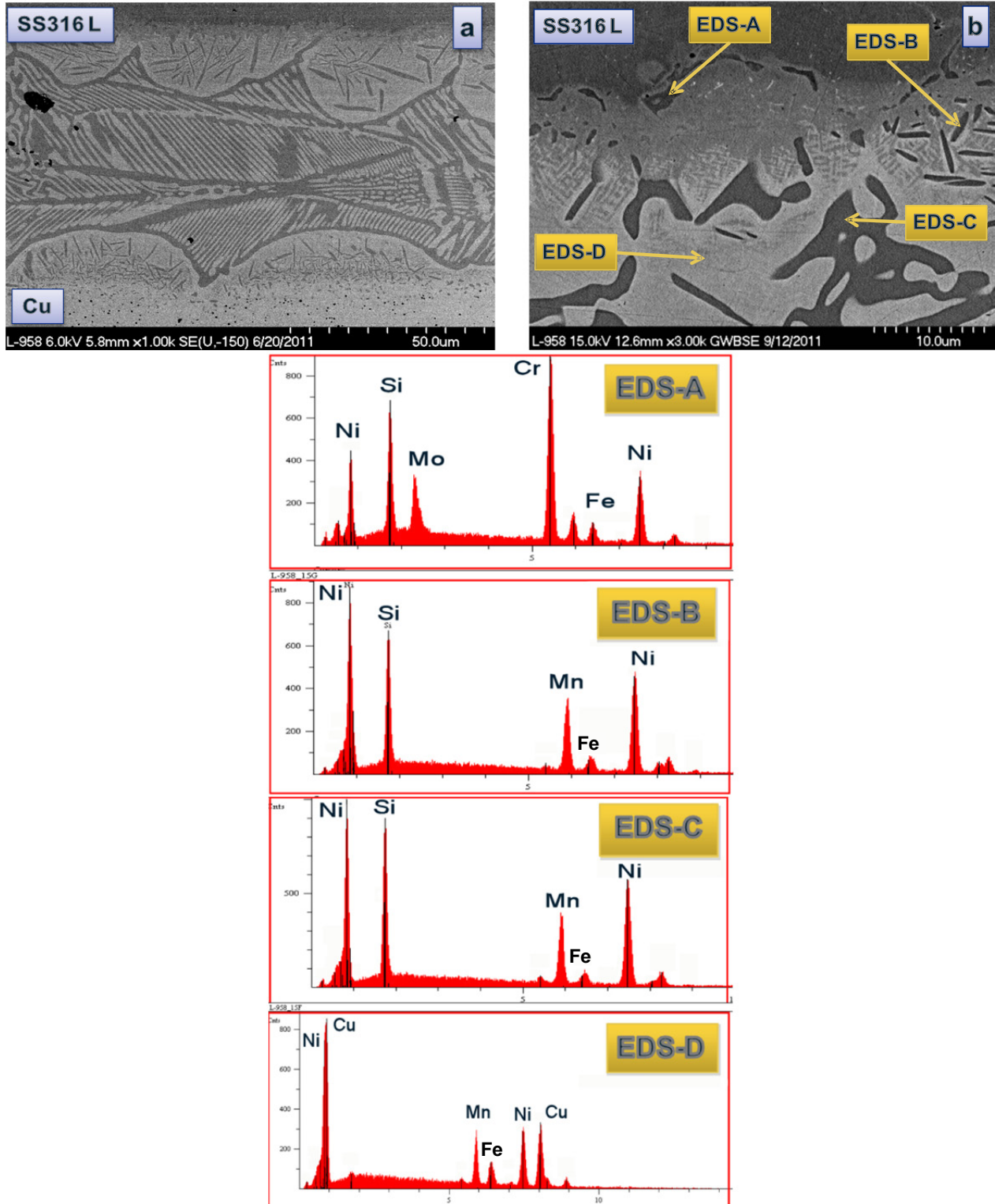
Figure 8.—(a) Low and (b) high magnification FESEM micrographs for sample aged for 1000 hr at 823 K (550 °C). Brazing alloy used is AMDRY 930. EDS analyses of second phases present next to SS/braze interface eutectic region.
