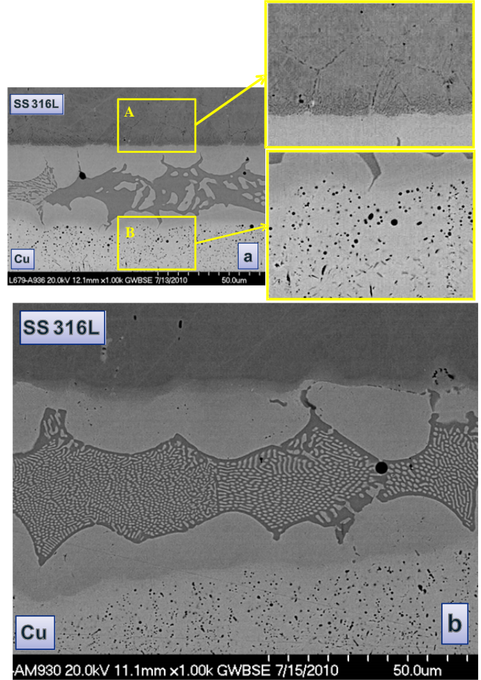
Figure 4.—FESEM micrographs of 316L stainless steel brazed to copper with (a) AMDRY 936 and (b) AMDRY 930. Eutectic phases formed at the center. Inserts in Figure 4a show (A) formation of chrome borides ( \text{CrB}_2 ) and (B) Manganese-copper (Mn-Cu) enriched particulates. No second phase precipitation occurred near the stainless steel / AMDRY 930 braze interface.
