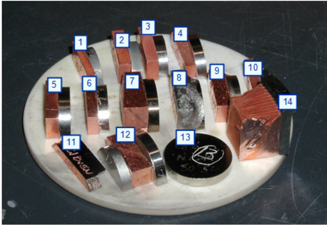
Figure 2.—Group of brazed samples aged at 823 K (550 °C) for 1000 hr in vacuum.
