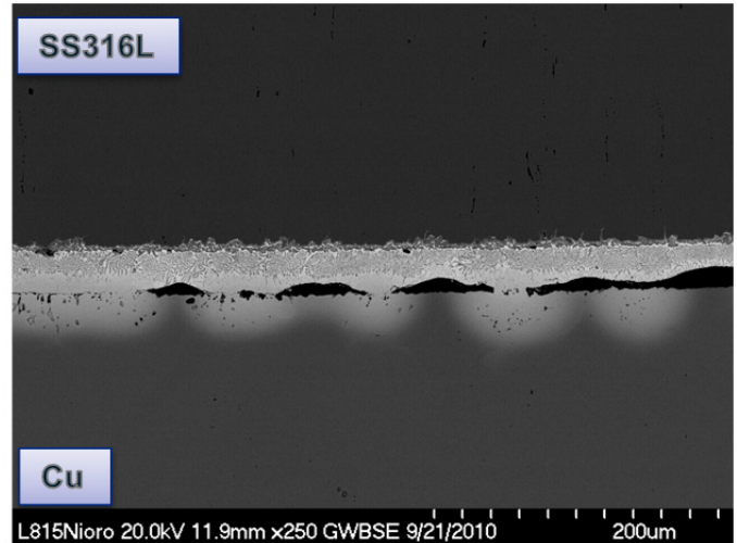
Figure 14.—Stainless steel brazed to copper using Niore braze alloy showing poor bonding.
