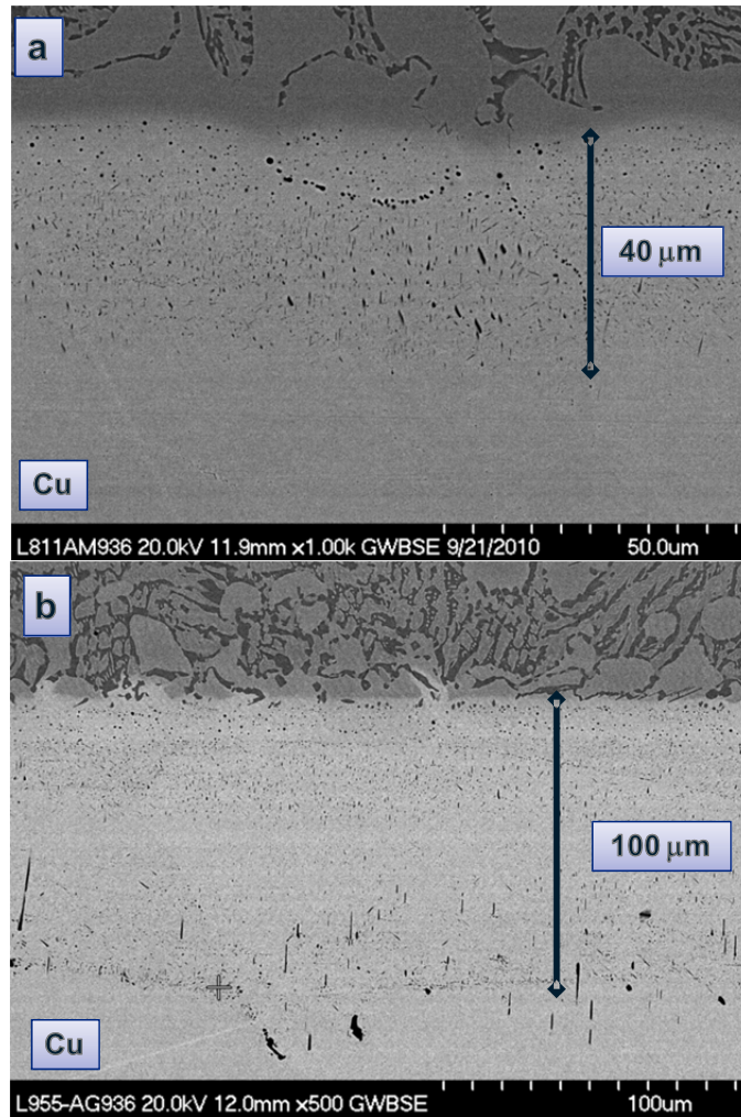
Figure 7.—FESEM Micrographs of the AM936 braze/copper interfaces in (a) as-brazed and (b) aged to 823 K (550 °C) for 1000 hr. Aging exposure resulted in an expansion of the region with Mn-Cu particulates.
