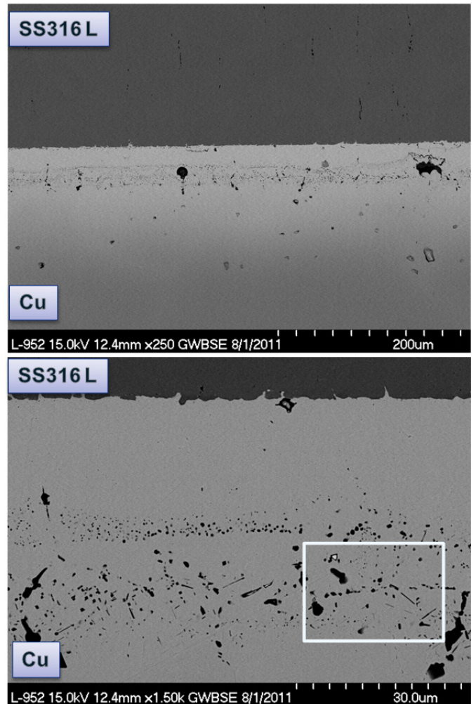
Figure 12.—Low and high magnification FESEM images of stainless steel brazed to Cu using a 50 Au – 50 Cu braze alloy after the aging heat treatment at 550 °C showing the formation of secondary phases at the braze/Cu interface.
