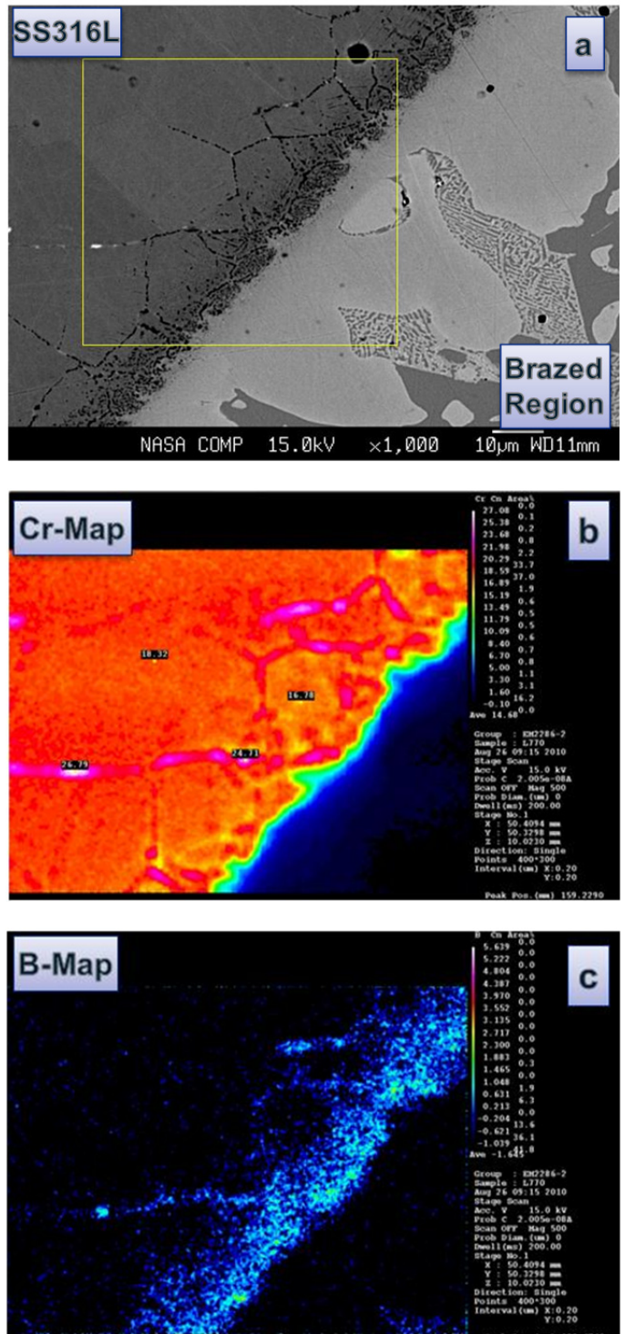
Figure 5.—Brazed SS316L to Cu with AMDRY 936 (a) Electron microprobe image and (b) and (c) Wavelength dispersive Spectroscopy (WDS) quantitative maps for Cr and B, respectively.
