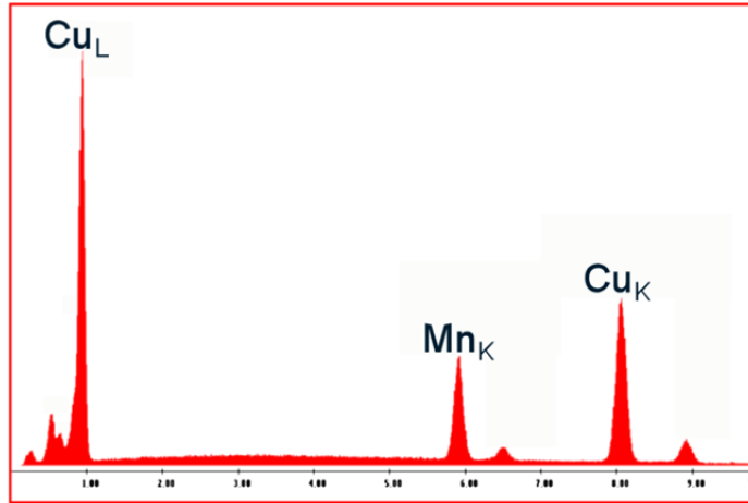
Figure 6.—Typical EDS spectrum of the fine Mn-Cu particulates formed on the Cu side of the as-brazed SS316L/Cu with AMDRY 930.
