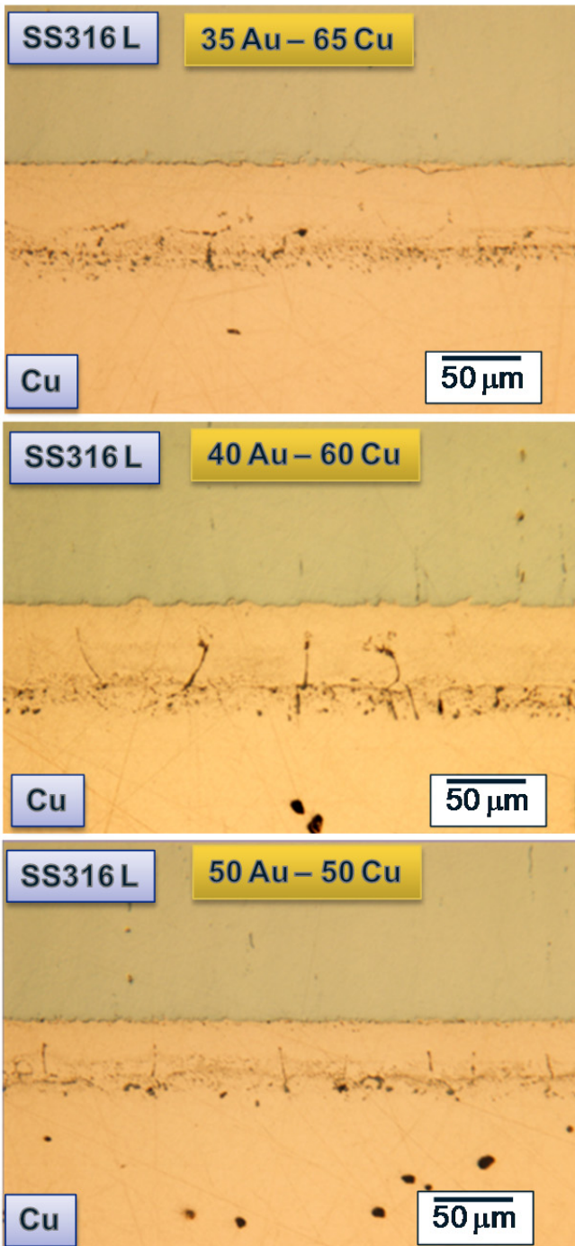
Figure 11.—Optical micrographs of stainless steel brazed to copper using gold-copper braze alloys after an exposure for 1000 hr at 550 °C showing some reactions at the braze/copper interface.
