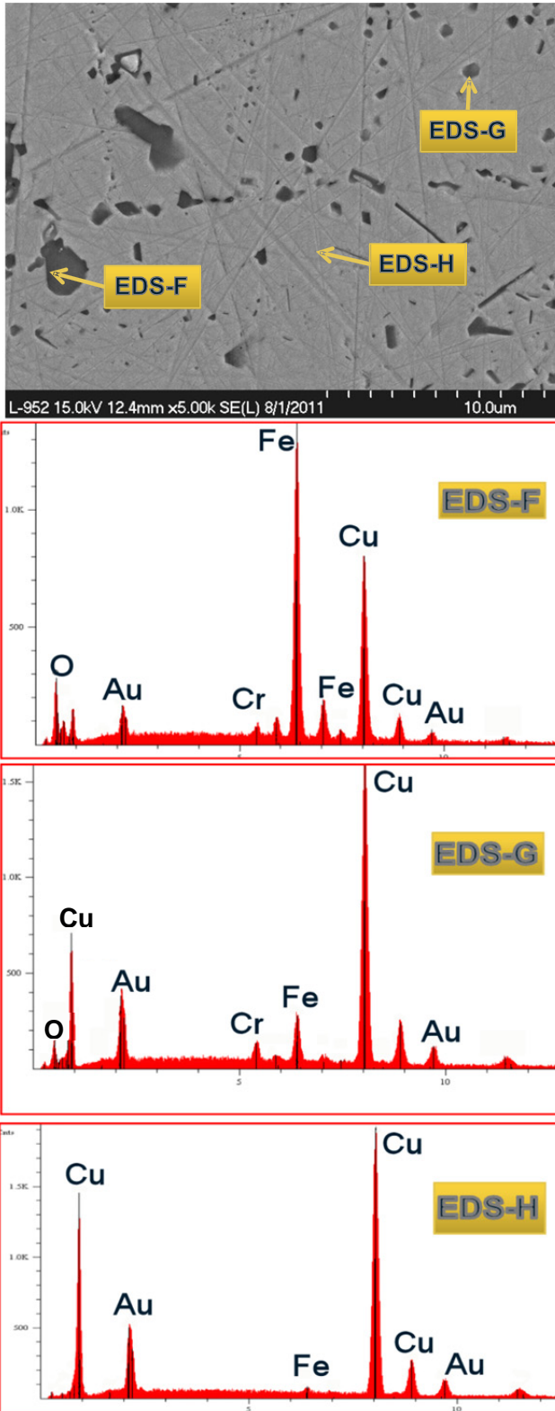
Figure 13.—Energy dispersive spectroscopy (EDS) spectra of main particulates and matrix detected in the selected region shown in Figure 12. Most precipitates are enriched in Fe (with some Cr) in addition to the presence of Cu and Au.
