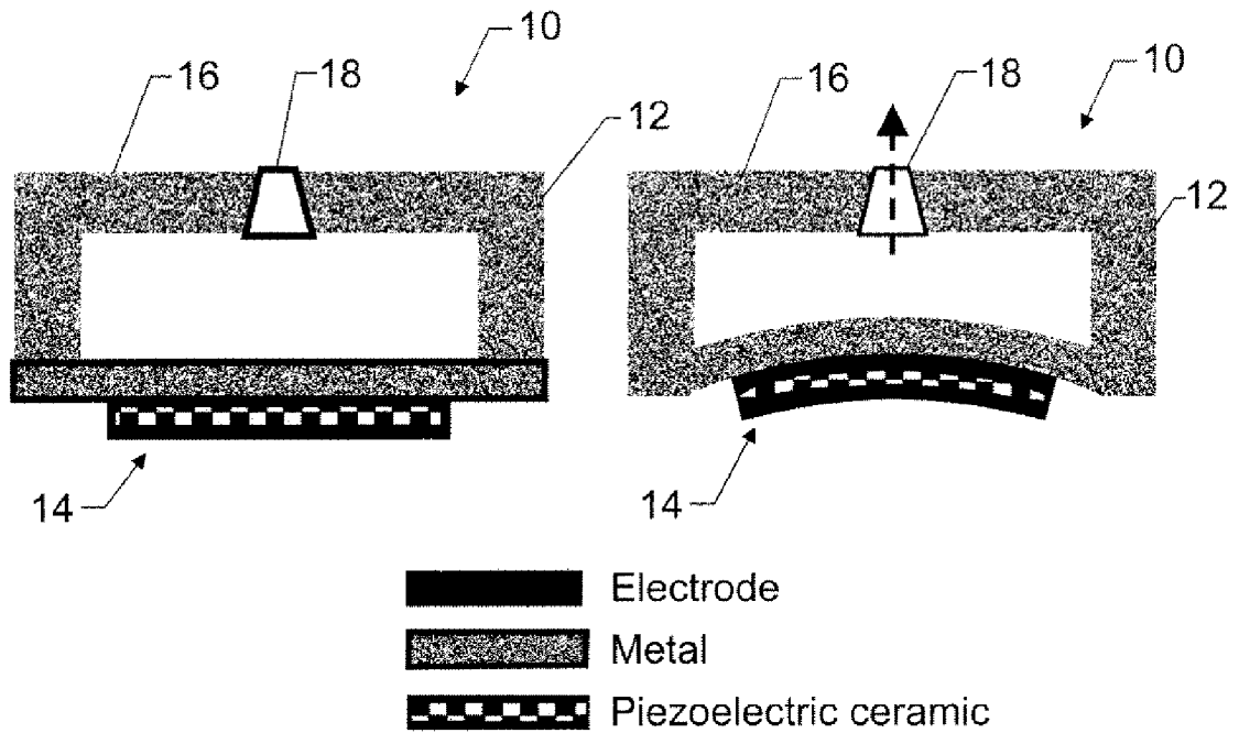
(b) A voltage applied
