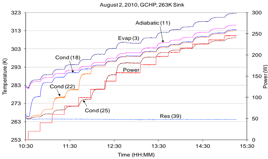
Figure 9 GCHP Heat Transport Test at 263K Sink Temperature
