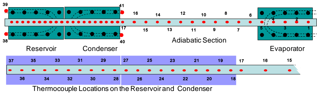
Figure 7. Thermocouple Locations for GCHP Test
