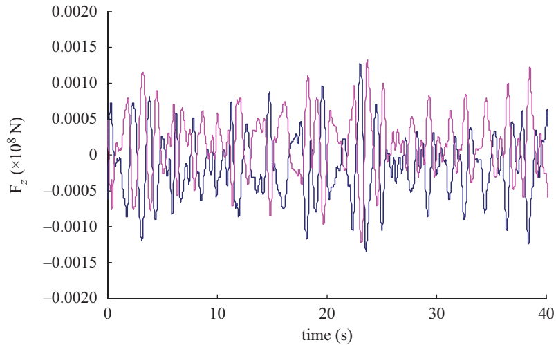
Figure 9. The numerical heave force \mathbf{F}_z^p and the restoring force \mathbf{F}_z^q (in the unit of 10^8 N) for the benchmark case in figure 7. Blue line, \mathbf{F}_z^p ; pink line, \mathbf{F}_z^q .
