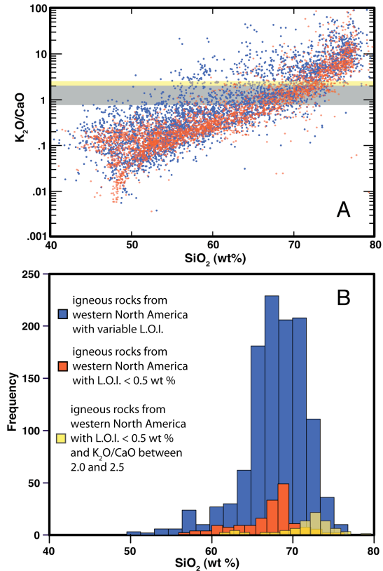
Fig. 2 (A) Plot of K 2 O/CaO vs SiO 2 with 4000 igneous rocks from the western US with variable L.O.I. and 2200 igneous rocks from the western US with L.O.I. < 0.5 % (all data extracted from www.navdat.org). Gray bar is the calculated K 2 O/CaO ratio of the parental material for granite clast from Apollo sample 14321 [15], and yellow bar is the upper estimate using the FAN age from [20] (B) Histogram of SiO 2 for data that fall in the gray bar and yellow bar in A.
