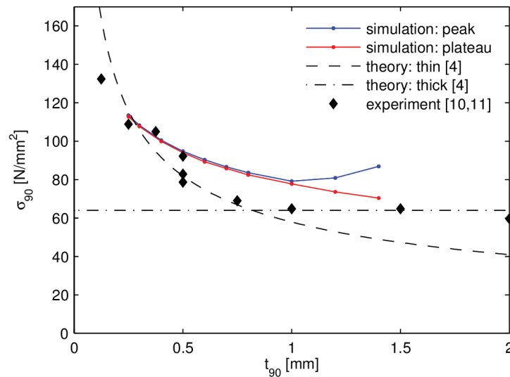
Figure 8. In situ effect as simulated with single element through the thickness of the transverse ply and constant interface stiffness.
