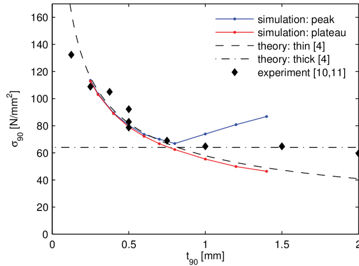
Figure 7. In situ effect as simulated with single element across the thickness of the transverse ply and with interface stiffness inversely proportional to the ply thickness.
