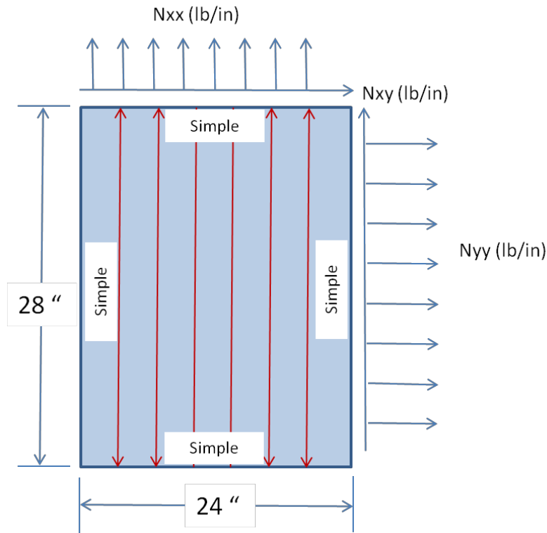
Figure 3. Skin panel geometry along with applied in-plane loads.
