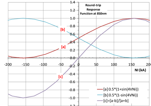
Figure 5. Reflective scheme response functions at 850 nm.
