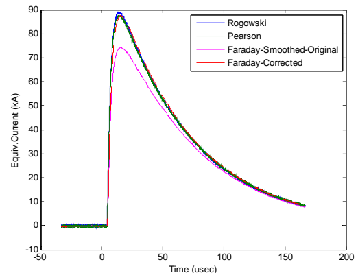
Figure 8. Faraday sensor comparison against reference sensors for a 90 kA current waveform.
