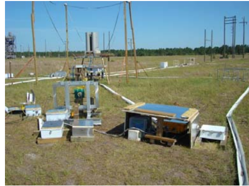
Figure 9. Field setup (right) located 12 m from the rocket launch pad.
