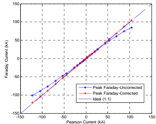
Figure 7. Faraday sensor's uncorrected and corrected (linearized) response curves.
