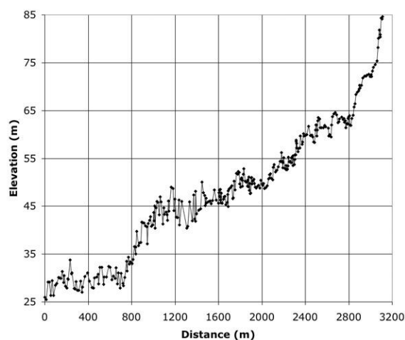
Figure 2. DGPS profile following the flow from the coastline (0 distance) going east to where the flow is on a slope typical of shield volcanoes.
