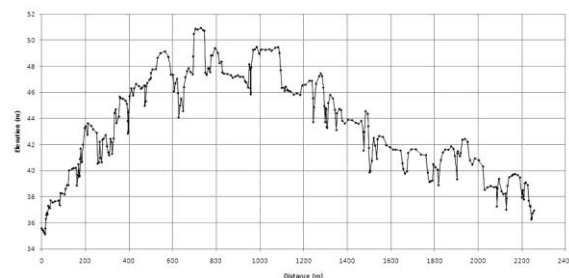
Figure 3. DGPS profile paralleling highway 11, going north to south, across the pāhoehoe flow ‘delta’. Several individual inflated flow lobes are evident.
