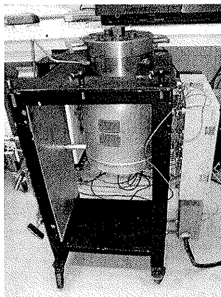
Figure 1: The Venus simulation chamber at NASA Goddard.
