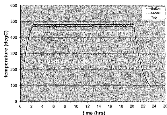
Figure 2: Temperature plot at 460^\circ\text{C} in the Venus simulation chamber
