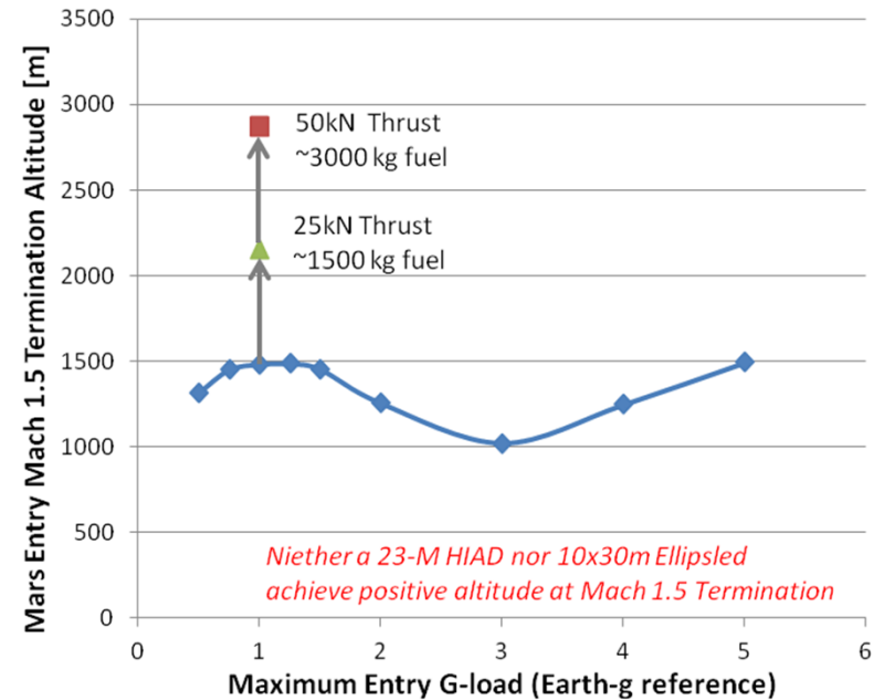
Mars Entry Performance for a slab delta with 60-degree sweep angle and 110000 kg entry mass.
