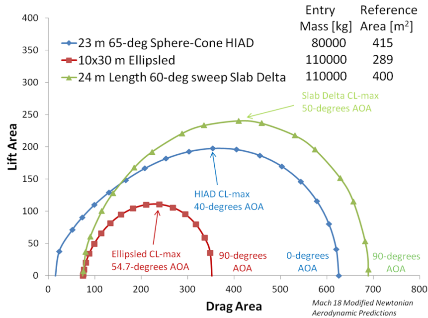
Drag polars for three hypersonic entry configurations based on modified Newtonian aerodynamics.
