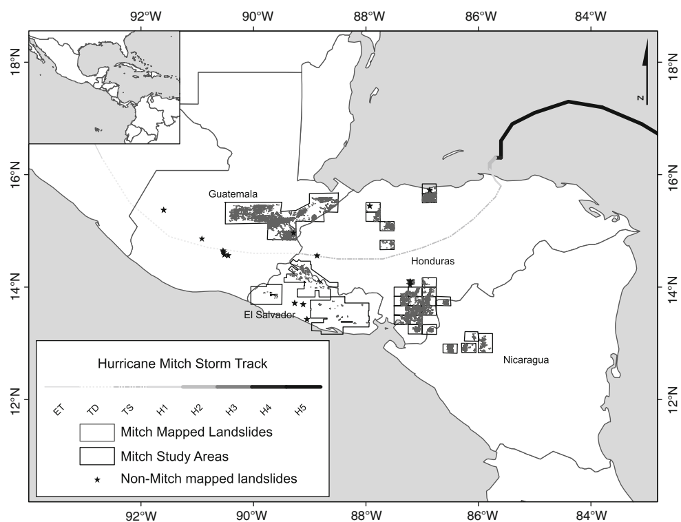
Fig. 3 Hurricane Mitch storm track and mapped landslide inventory study areas. The total inventory contains over 24,000 landslides, covering a total study area of 35,474 sq km. The 19 landslide events not associated with Hurricane Mitch (non-Mitch landslides) are extracted from the global landslide catalog described in Kirschbaum et al. (2009b)
