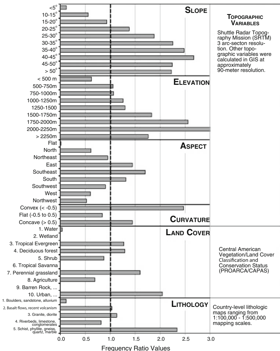
Fig. 4 Surface observable data, binned categories, and corresponding frequency ratio values used in the regional susceptibility evaluation. Frequency ratio values exceeding the black dashed line (Fr = 1), suggests that as the value diverges from 1, there is a more pronounced relationship between the landslide and total pixel area
