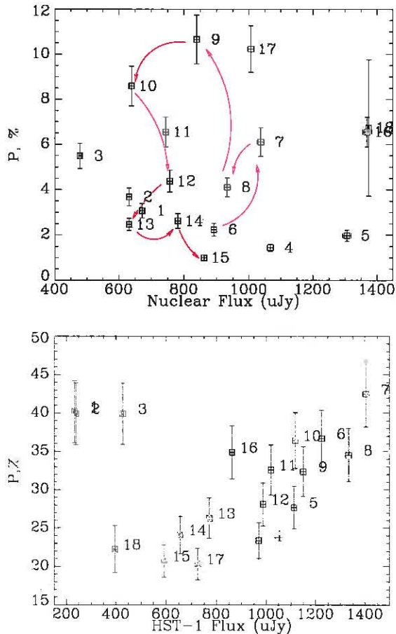
FIG. 3.— Graphs of fractional polarization versus flux for the core (top) and HST-1 (bottom). The observation epochs have been labelled sequentially. Notice that for HST-1, epochs 4-18 display a very strong correlation between the flux and polarization, whereas the behavior for the nucleus is very different, with a ‘loop’ seen between epochs 9-15, but otherwise no organized pattern.
