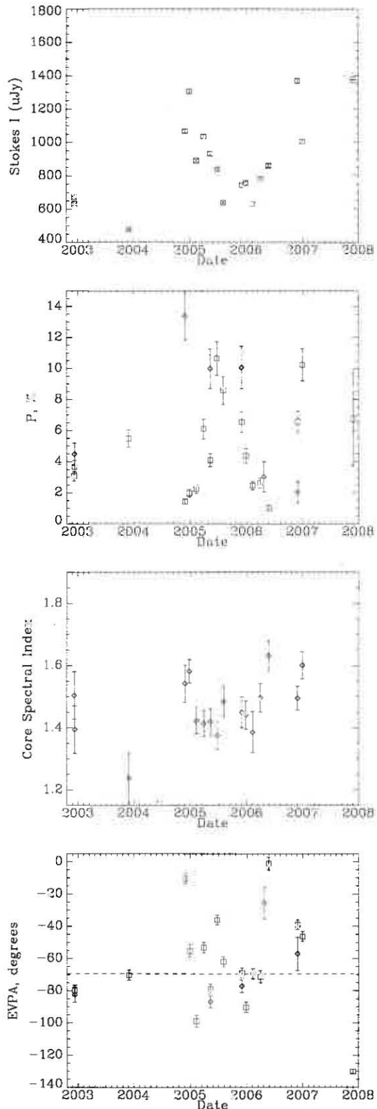
FIG. 1.— Variations in Total flux (i.e., Stokes I), fractional polarization, spectral index and EVPA, are plotted for the nucleus of M87. A dashed line in the EVPA panel reflects the jet PA. The F606W observations are plotted as squares, while in the second and fourth panel the F330W polarimetry is plotted as diamonds. See §3.2 and 4 for discussion.
