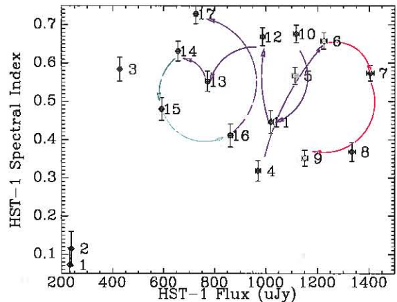
FIG. 4.— The evolution of \alpha_{UV-O} versus flux for knot HST-1. Each epoch has been labelled sequentially, as in Figure 3. Notice the strong ‘looping’ behavior during the maximum of the flare in HST-1, as well as after (green and red arrows). See §§4, 5.1 for discussion.
