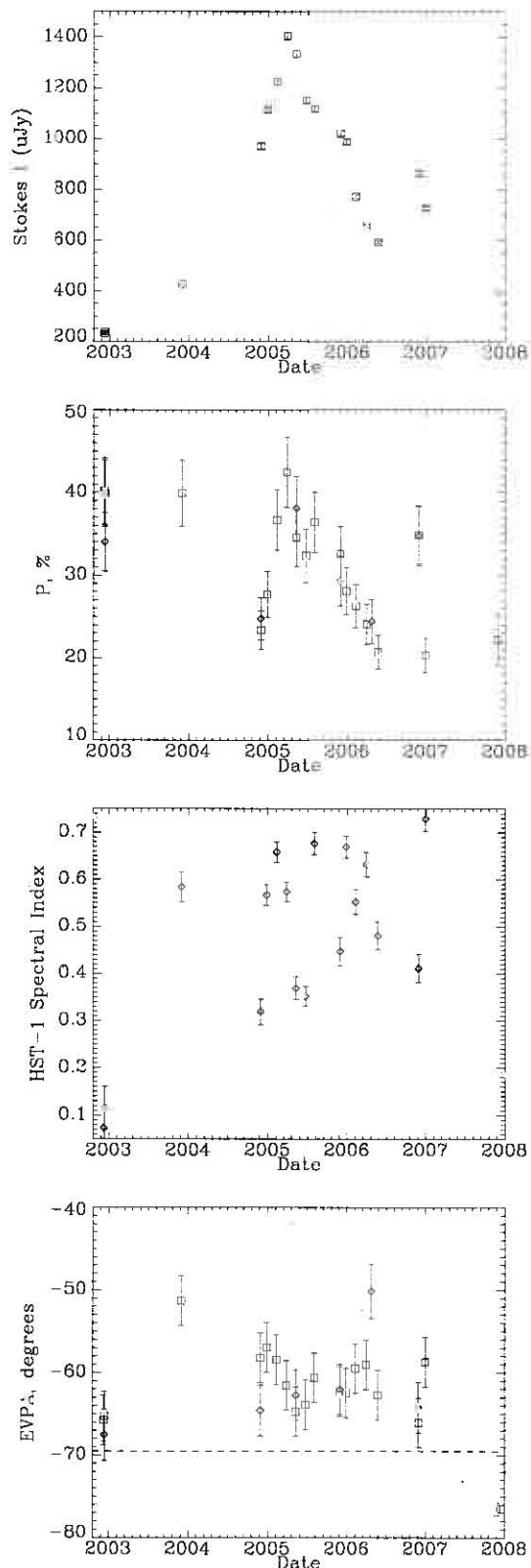
FIG. 2.— Variations in Total flux, fractional polarization, spectral index and EVPA, are plotted for knot HST-1. A dashed line in the EVPA panel reflects the jet PA. The F606W observations are plotted as squares, while in the second and fourth panel the F330W polarimetry is plotted as diamonds. See §3.2 and 4 for discussion.
