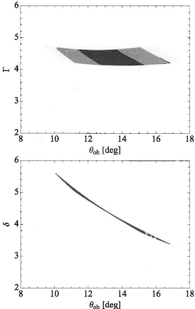
FIG. 6.— Allowed values of beaming parameters for our shock model of knot HST-1. At top, we show the allowed range for the Lorentz factor \Gamma and viewing angle \theta_{ob} , while at bottom, we show the corresponding range for the Doppler factor \delta plotted against viewing angle \theta_{ob} . In both panels, light gray colors refer to spectral indices \alpha = 0.45 , gray colors refer to \alpha = 0.5 , and black colors refer to \alpha = 0.55 . See §§5.1, 5.2 for discussion.
