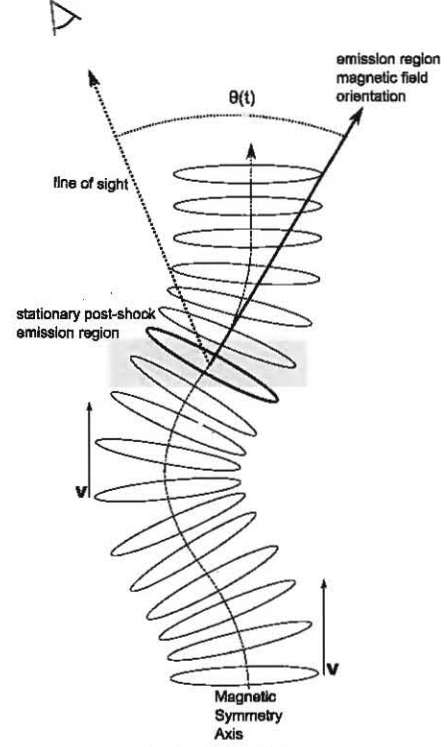
FIG. 5.— Schematic of the helical distortion model illustrated with toroidal loops of magnetic field. As shown by the velocity vectors (labeled by \mathbf{v} ), the velocity field is uniformly directed despite the kinked jet. As the kinked region of the jet propagates through the standing shock's emission region (gray region), the orientation of the magnetic field with respect to the line of sight changes with time. This change in orientation is parametrized as \theta'(t) in equation (7). The effects of shock compression, the poloidal magnetic field and the change in the magnetic pitch angle, \psi'(t) , are not shown.
