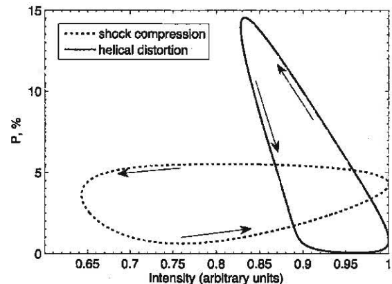
FIG. 7.— Illustrated here is a theoretical counter-clockwise I - P loop for the helical distortion model (solid) and the variable shock compression model (dotted). The values used in the shock compression model are: (\beta_{u,0}, A_\beta, \omega_\beta, \phi_\beta) = (0.78, 0.03, 1, -\pi/2) and (\xi_0, A_\xi, \omega_\xi, \phi_\xi) = (0.78, -0.5, 1, 0) . For the helical distortion model, (A'_\theta, \omega_\theta, \phi_\theta, \theta'_{ob}) = (1.5, 1, 0, \pi/2) and (A'_\psi, \omega_\psi, \phi_\psi, \psi'_0) = (0.05, 2, 0, 1.03) and \delta = \sin \theta'_{ob} / \sin 15^\circ \approx 3.86 . For both models, \theta_{ob} = 15^\circ and \alpha = 1.5 were used.
