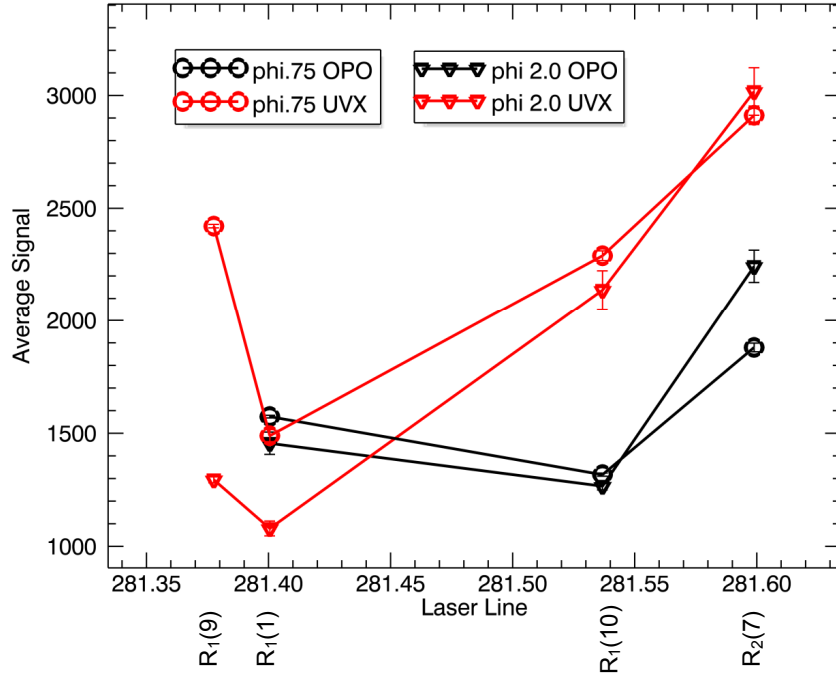
Figure 7.—Average PLIF signal versus the OH excitation line wavelengths for both lasers and both equivalence ratios. R 1 (9) = 281.3776 nm, R 1 (1) = 281.4005 nm, R 1 (10) = 281.5368 nm, and R 2 (7) = 281.5989 nm.
