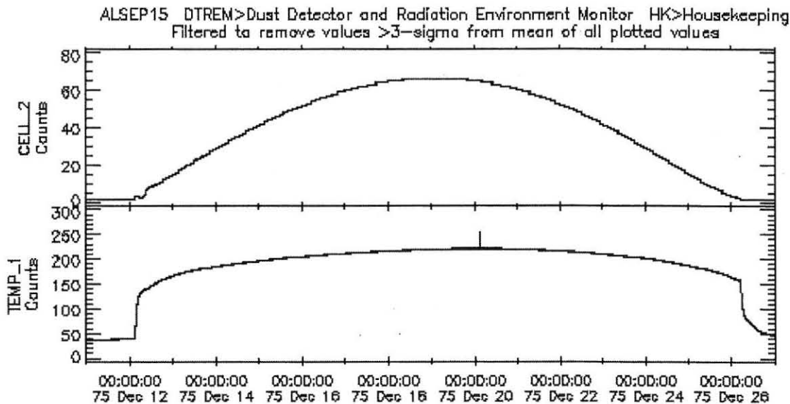
Figure 1 – Sample output of the raw telemetry data from the Apollo 15 DTREM showing solar cell and temperature counts measured in December 1975.
