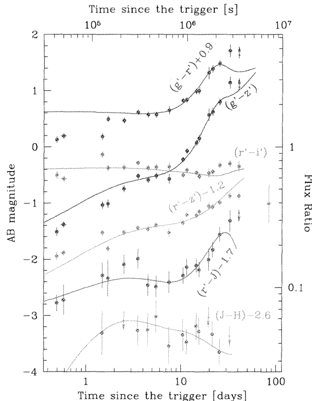
Fig. 6. Colour curves corrected for host-galaxy extinction and afterglow-subtracted. Filled circles represent detections in both filters and arrows are upper limits derived from detections in one of the two bands. Solid lines represent the colour evolution of SN 1998bw derived from the light-curve fits in Sect. 4.3. For clarity, error bars do not include the systematic error in A_{V,\text{host}} and for the last epoch, upper limits are not shown.
