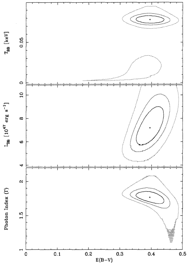
Fig. 3. Contour plots for the best-fit parameters from the modelling of the second epoch. From the outer- to the innermost contours, the red, red, and black lines are 3, 2, and 1\sigma contours, respectively. The tail at low \Gamma in the bottom panel is caused by numerical inaccuracies.
