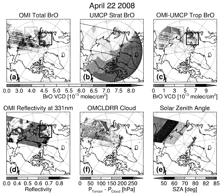
Fig. 5. Measured total vertical column BrO, reflectivity, and cloud pressure for OMI orbit 20050 at 03:23 UTC on 22 April 2008 as well as calculated stratospheric column BrO for the time of OMI overpass and the inferred tropospheric residual column BrO. The panels highlight reduced tropospheric BrO over low albedo surfaces (black box) and in the presence of shielding clouds (orange box). See text for more details and discussion.
