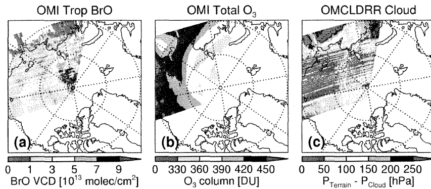
Fig. 12. (a) OMI tropospheric BrO VCD; (b) OMI total ozone column; (c) terrain minus cloud pressure for OMI orbit 19976 on 17 April 2008.
