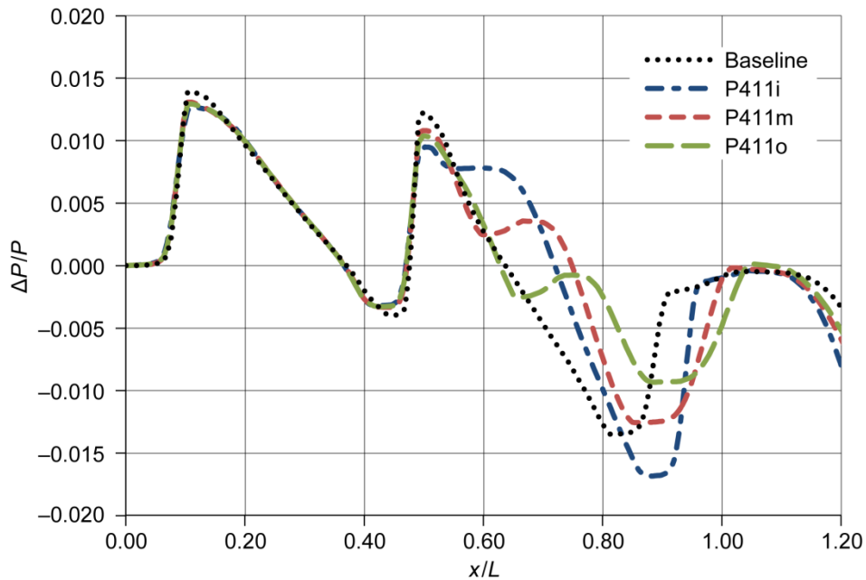
Figure 14.—Swept wing-body pressure profiles ( \Delta P/P ) for plug nozzle configurations, NPR = 8 , h = 3 L_V below vehicle.
