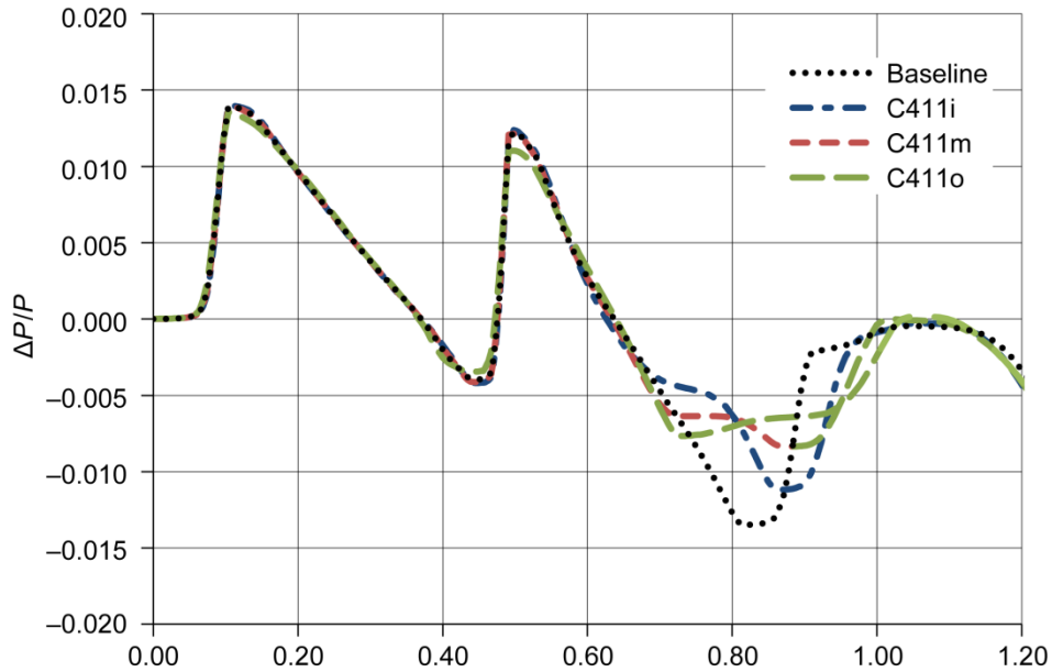
Figure 13.—Swept wing-body pressure profiles ( \Delta P/P ) for convergent-divergent nozzle configurations, NPR = 8 , h = 3 L_V below vehicle.
