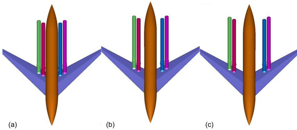
Figure 9.—Cart3D model of the swept wing-body model with convergent-divergent nozzles installed, (a) inner, (b) middle, and (c) outer engine mounting positions.
