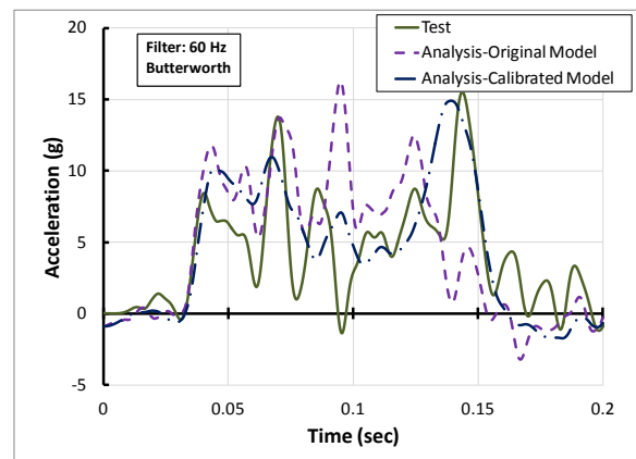
Figure 26. Pilot floor vertical acceleration, crash test with DEA
