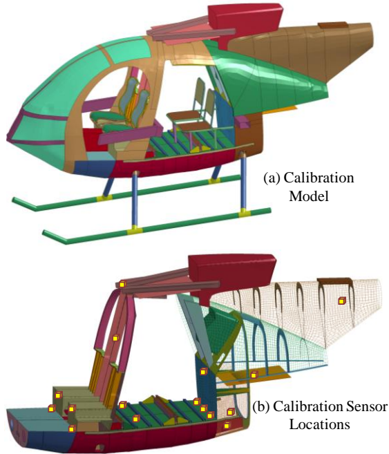
Figure 17. Calibration FEM
