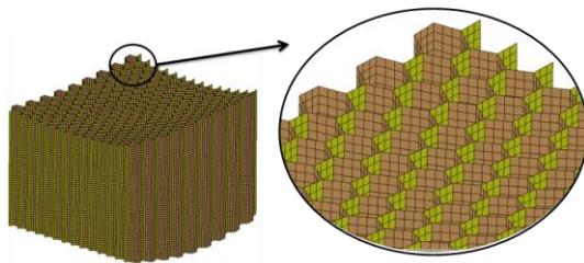
(a) Shell Based DEA FEA
