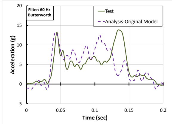
Figure 11. Comparison of test and analysis, passenger floor vertical acceleration, crash test with DEA
