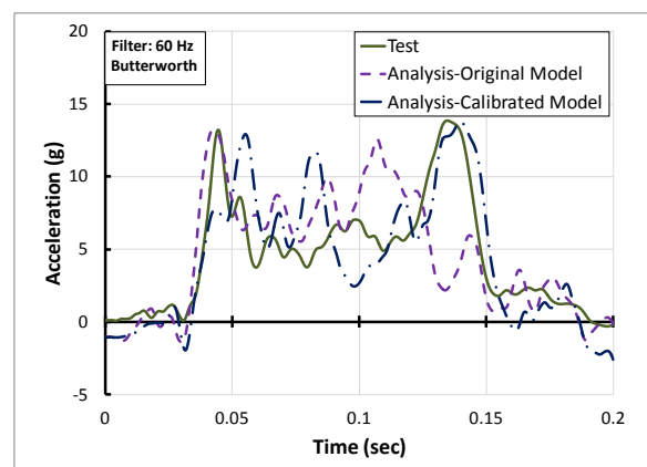
Figure 27. Passenger floor vertical acceleration, crash test with DEA
