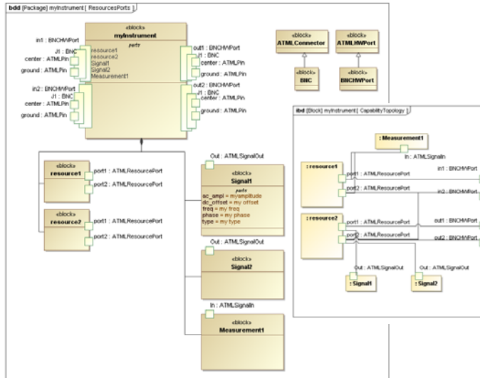
Figure 10. BDD and IBDD Techniques for Representing Capabilities and Resources
