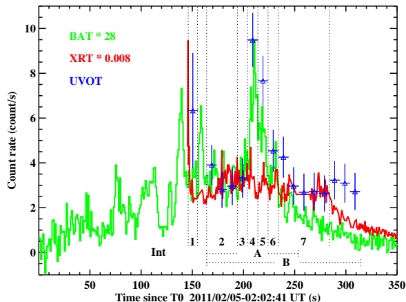
Fig. 1.— Prompt light curves of GRB 110205A from Swift BAT ( green ), XRT( red ) and UVOT( blue ). Arbitrary scale. For the UVOT data, the first data point is in v , but has been normalized to white band, the rest of the data are in white . The vertical lines partition 9 intervals for constructing the prompt spectra, where Int A and B are averaged ones.
