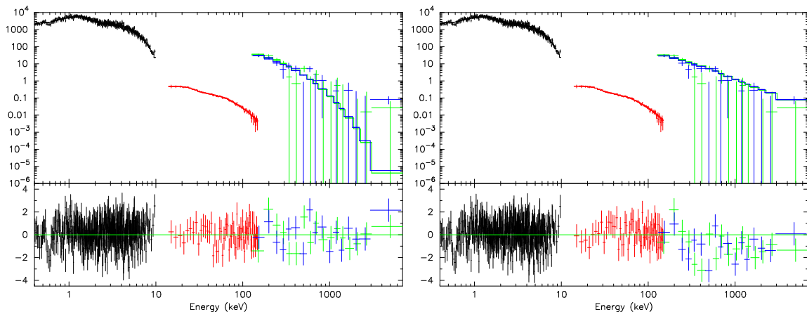
Fig. 2.— The XRT (black), BAT (red) and WAM (green and blue) count spectra of intB with the bandcut model (left panel) and the standard Band function (right panel) fit. The improvement using bandcut model can be easily seen in the residual panel at the bottom.
