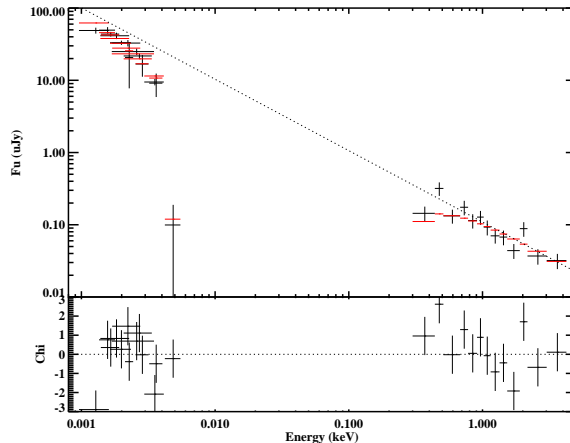
Fig. 7.— Afterglow SED of GRB 110205A at 35 ks. Black data are the observed data, red data are the predicted value from the model. Dotted line is the original power-law model without absorption or extinction.
