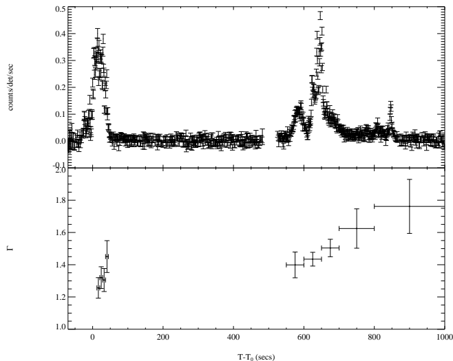
FIG. 1.— BAT count rates (upper panel) and photon index evolution (lower panel) of GRB 110709B. The spectral model is a simple power law.
