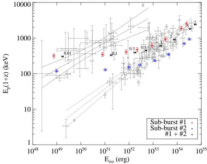
FIG. 11.— E_p - E_{iso} plot made by putting the double burst at different assumed redshift z_x . Red: the first sub-burst. Blue: the second sub-burst. Black: the whole double burst. For each group of three points (red, blue and black), the nearest number indicates the corresponding assumed redshift z_x .
