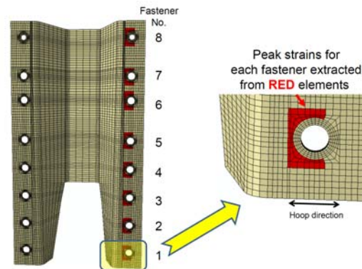
Figure 21. Selected element subgroups for strain recovery during the assembly simulation – red elements denote the fastener element group used to extract peak strain values near each fastener.
