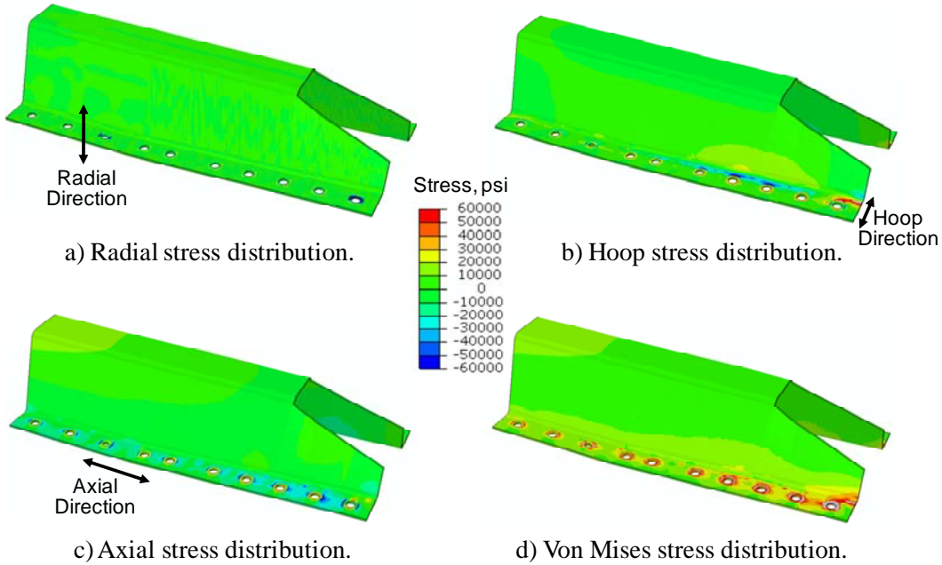
Figure 25. Stringer stress contours by component with flight loading applied for the flat-foot configuration with radius blocks. Stress values plotted as gray exceed the maximum tensile value, and values plotted as black exceed the maximum compressive value.
