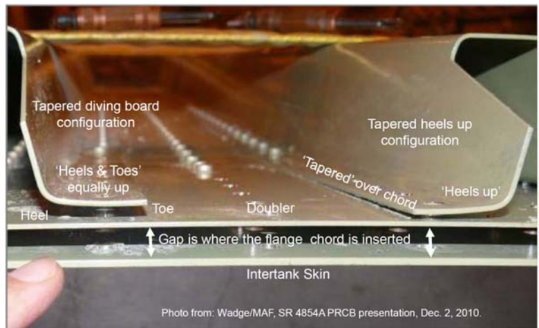
Figure 7. Various stringer-foot imperfections. Photograph courtesy of Mr. G. Wadge/LM-ET.
