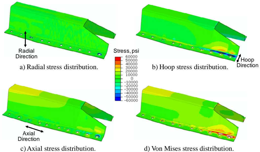
Figure 24. Stringer stress contours by component at 3620 seconds after starting tanking for the flat-foot configuration with radius blocks. Stress values plotted as gray exceed the maximum tensile value, and values plotted as black exceed the maximum compressive value.
