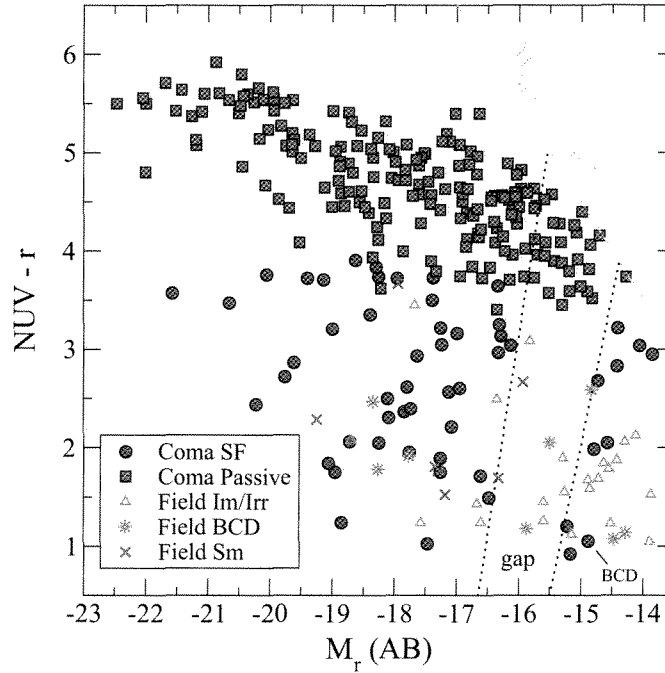
FIG. 13.— NUV- r vs. M_r CMD comparing Coma member galaxies and dwarf star forming galaxies located in the local field/group environment (Hunter et al. 2010). Coma members are separated into passive (red squares) and star forming galaxies (blue circles); a candidate BCD galaxy in Coma is identified in the bottom right corner of the diagram. Field galaxies are separated by morphology as Sm (magenta Xs), BCD (green asterisks), and Im/Irr galaxies (brown open triangles). We re-reddened the field galaxies by the internal dust prescription used in Hunter et al. (2010) and converted their optical V -band to the SDSS r -band based on typical SEDs for these galaxies. The gray dashed line shows the NUV magnitude limit of this study and black dotted lines enclose the gap. Im/Irr galaxies are the majority galaxy type in the field starting at the gap (and extending to fainter magnitudes), and hence are the likely candidate for the missing dwarf star forming galaxies in Coma.
