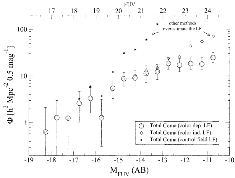
FIG. 9.— Comparison of Coma FUV LFs that were measured using three different techniques. Large gray-filled circles show the FUV LF measured using the color-dependent spectroscopic completeness method (the method adopted for this study). The two alternative LFs are measured using the color-independent completeness method (diamonds) and the subtraction of a control field (asterisks). The alternative methods clearly overestimate the LF and result in steeper faint-end slopes.
