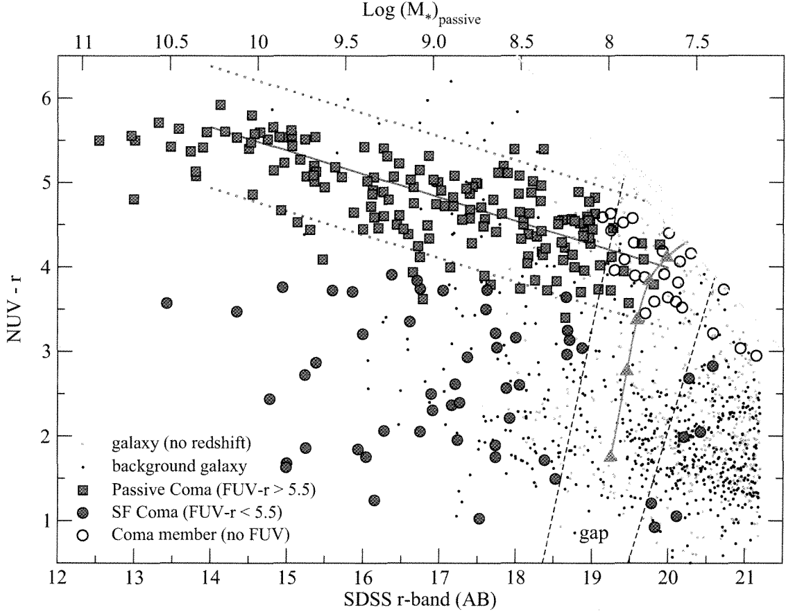
FIG. 5.— NUV-optical CMD for all galaxies in our sample. Orange dots are galaxies that lack spectroscopic redshifts, black dots are confirmed background galaxies, and confirmed Coma members are shown as large symbols (red squares=passive; blue circles=star forming; black open circles=no FUV color information). We have spectroscopic redshift coverage across the full magnitude-color space. A linear fit to passive Coma member galaxies (red solid line) and the 2\sigma scatter (red dotted lines) are shown. The majority of Coma members without FUV colors are passive galaxies as they are located inside the 2\sigma scatter. The top x-axis gives the average stellar masses for passive Coma member galaxies as measured in this study ( \text{Log } M_* = 16.364 - 0.435 \times r ; Section 3.2); SF galaxies are \sim 0.5 mag brighter in the r -band for a given stellar mass. The black dashed lines enclose a “gap” in the CMD that is void of confirmed Coma member galaxies. Inside the gap, the thick green line is the path that a dwarf SF galaxy in Coma would follow after a rapid 100 Myr quenching event (see Section 3.3); the line spans 4 Gyr from the onset of quenching and triangles show the model after 0, 0.25, 0.5, 1, and 2 Gyr. The gray long-dashed line is our chosen magnitude limit at \text{NUV}=24.5 .
