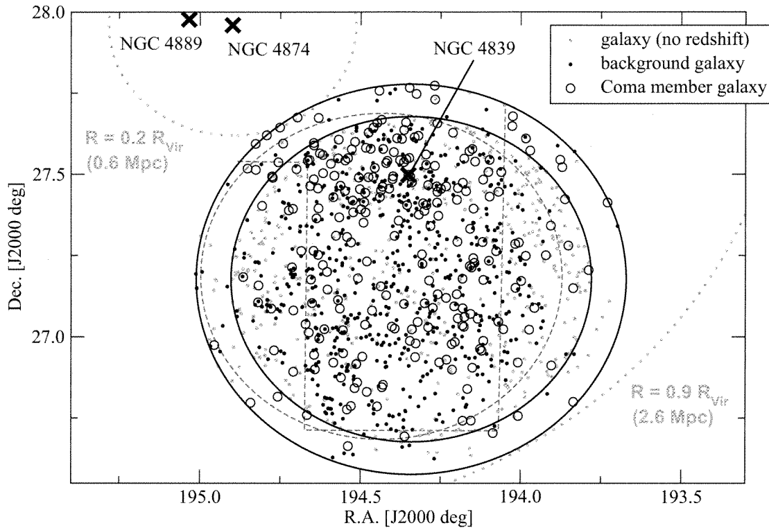
FIG. 1.— Location of our GALEX field at the Coma-3 infall region of the Coma cluster. Bold Xs mark the three largest galaxies in Coma (NGC 4889, 4874, 4839). Concentric circles (black) show the inner 0^{\circ}.5 and 0^{\circ}.6 GALEX FOV which span cluster-centric distances of R = 0.2 and 0.9 R_{\text{vir}} (blue dotted lines). GALEX coverage extends to \text{NUV}=24.5 and \text{FUV}=24.5 mag inside the inner circle, and \text{NUV}=21.0 and \text{FUV}=21.0 mag inside the outer circle. Spatial locations are shown for the 1297 galaxies in our trimmed catalog (see Section 2.4), separated into three subsets that include galaxies that lack redshifts (458 orange dots), confirmed background galaxies (591 black dots), and confirmed Coma member galaxies (248 open black circles). SDSS photometric and spectroscopic coverage is available across the full GALEX FOV. Deeper spectroscopic redshift coverage is available from surveys performed with MMT-Hectospec (dashed red circle) and WHT (dashed red rectangular regions; Mobasher et al. 2001).
