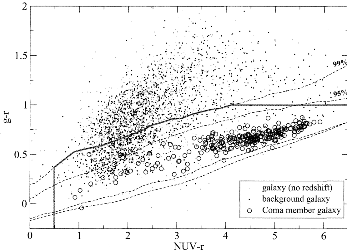
FIG. 2.— UV-optical color-color diagram for galaxies in the full GALEX /SDSS catalog. The sample is separated into three subsets that include galaxies that lack spectroscopic redshifts (orange dots), spectroscopically confirmed background galaxies (black dots), and confirmed Coma member galaxies (open black circles). Dashed lines trace the bi-variate density distribution of \sim 100,000 model SEDs (from Salim et al. 2007, see Section 2.3 for details) that are used to identify the color space where Coma member galaxies are expected; the inner and outer contours enclose 95% and 99% of the models, respectively. We use the thick red line to exclude 1828 obvious background galaxies that are shifted above this cutoff owing to K-corrections and keep the 1297 galaxies located below the line. The red sequence of cluster member galaxies is clearly visible at UV-optical colors redder than \text{NUV-}r \approx 3.5 .
