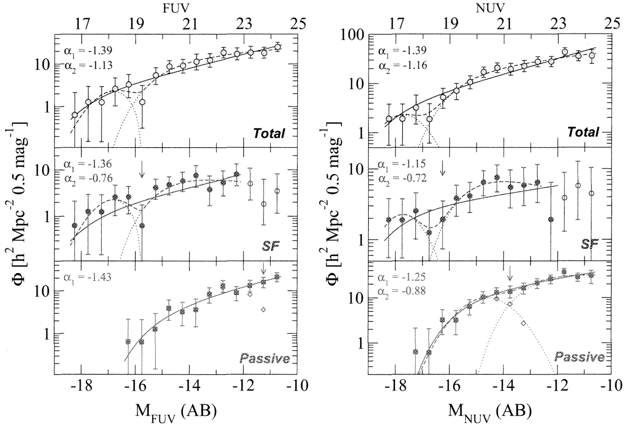
FIG. 10.— Fits to the Coma FUV and NUV LFs for the total galaxy population (top panels), star forming galaxies (middle panels), and passive galaxies (bottom panels). In each panel, the solid line shows the best-fit Schechter function. Dotted lines show the separate components of the Gauss-plus-Schechter models with dashed lines showing the sum of both functions. The faint-end slopes for the Schechter ( \alpha_1 ) and Gauss-plus-Schechter ( \alpha_2 ) fits are listed in the upper left corner of each panel. The full list of fitted parameters is given in Table 2. Arrows in the bottom two panels indicate the magnitudes where dwarf galaxies ( M_r > -18.5 ) become the majority population; the Schechter component of the Gauss-plus-Schechter model is essentially a fit to the dwarf galaxy population for the bottom two panels. Diamonds in the bottom panels show the LF for normal passive galaxies ( M_r < -18.5 ). We did not fit a Gauss-plus-Schechter model to the FUV passive LF as dwarf galaxies are the majority in only the last few magnitude intervals. The Gauss-plus-Schechter models, in addition to providing a more physical interpretation of the SF and passive LFs (see Section 4.1.2), are a better match to the shapes of the total and SF LFs.
