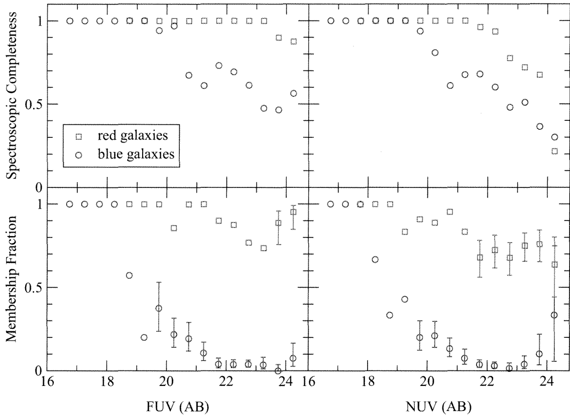
FIG. 7.— Properties of the spectroscopic redshift coverage at FUV (left panels) and NUV (right panels) wavelengths. The spectroscopic completeness - the fraction of all galaxies with spectroscopic redshifts - is shown in the top panels ( N_s/N_p ). The membership fraction - the fraction of galaxies with redshifts that are cluster members - is shown in the bottom panels ( N_c/N_s ). Measurements are performed separately for blue/red galaxies using the color separation defined in Figure 6. The uncertainties are binomial errors from the formalism in Gehrels (1986); error bars are shown only at magnitudes where we use membership fractions to measure the LF (i.e., where the spectroscopic completeness is less than 100%). The top panels indicate that red galaxies have higher spectroscopic completeness as compared to blue galaxies, and bottom panels show that a significantly higher fraction of red galaxies are Coma members. Given the color dependence of the spectroscopic redshift coverage, we construct the Coma UV LF as a summation of the separate blue/red LFs in order to avoid systematic color selection effects.
