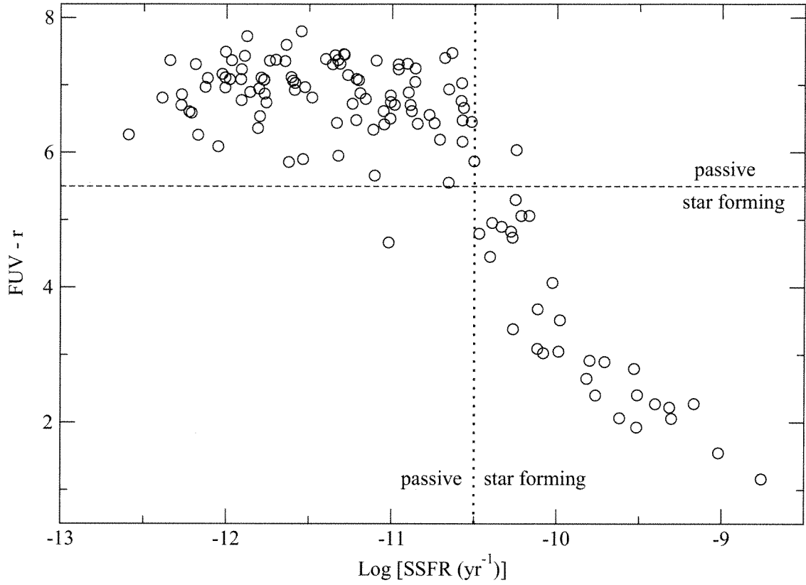
FIG. 3.— FUV- r color vs. specific star formation rate (SSFR) for Coma member galaxies. SSFRs are taken from the MPA-JHU SDSS value-added catalog (e.g., Brinchmann et al. 2004) which is limited to galaxies brighter than r \approx 17.8 mag. The vertical dotted line indicates the typical separation in SSFR for galaxies classified as star forming or passive (e.g., Salim et al. 2007). The diagram shows that FUV- r color allows for a similar separation of SF and passive galaxies in Coma with a dividing line at FUV- r=5.5 mag (horizontal dashed line).
