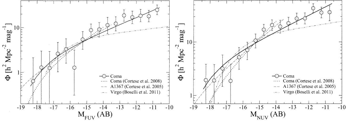
FIG. 11.— FUV and NUV LFs of the Coma cluster (gray filled circles; black solid line) compared to previous GALEX LFs in Coma (black dotted), A1367 (green dashed), and Virgo (red dashed-dot). The comparison LFs were derived from the published Schechter parameters and normalized to the integral of our Coma LF at magnitudes brighter than M_{\text{UV}} = -14 . The shapes of the LFs are similar at bright magnitudes despite their different environments and cluster-centric coverage (see Section 4.2.1). Although our Coma LFs agree with Cortese et al. (2008) across magnitudes where there is overlap ( M_{\text{UV}} < -14 ), our faint-end slopes are much shallower owing to a flattening of the Coma UV LFs at faint magnitudes (especially in the NUV band).
