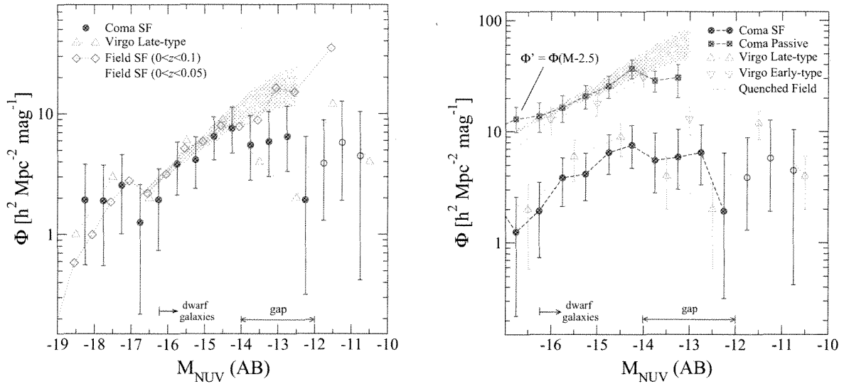
FIG. 12.— ( Left ) NUV LF for star forming galaxies in Coma (blue circles) as compared to the Virgo cluster (orange triangles; Boselli et al. 2011) and the field environment (green diamonds; Treyer et al. 2005). The gray shaded region is another field LF that we derived from previous SDSS and GALEX LFs (see Section 4.2.1; Blanton et al. 2005; Wyder et al. 2007). The bottom of the diagram shows the magnitude ranges associated with dwarf galaxies in Coma and the gap. The field LFs were normalized to the average of Virgo and Coma at magnitudes brighter than M_{\text{NUV}} = -14 . The Virgo LF is shown at its true value. The Coma and Virgo LFs have similar shapes and show the same turnover at M_{\text{NUV}} = -14 , whereas the field LFs continue to rise at faint magnitudes. This suggests that external processes related to the cluster environment are more efficient in disrupting fainter (lower mass) galaxies. ( Right ) Same as the left panel but now including passive galaxies in Coma (red squares) and Virgo (orange triangles - pointing down). We have shifted the passive LFs to brighter magnitudes (2.5 mag) to match the typical color separation of star forming and passive galaxies at the turnover. The matched LFs follow similar shapes and show the same turnover, suggesting that the dwarf passive population in each cluster may be built from recently quenched star forming galaxies. The shaded region models the expected distribution of dwarf passive galaxies for a field galaxy population that is quenched but not destroyed (see Section 4.2.1); the divergence of the passive LFs relative to this model is consistent with an infall population that has a turnover prior to reaching the cluster virial radius.
