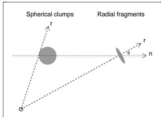
Figure 1. Schematic of photon of direction \mathbf{n} impacting a spherical clump and a radially oriented ( \mathbf{r}/|r| ) shell fragment. The former gives an isotropic effective opacity whereas the latter gives an anisotropic effective opacity, since the projected surface area depends on direction cosine \mu \equiv \cos \theta = \mathbf{n} \cdot \mathbf{r}/|r| .
