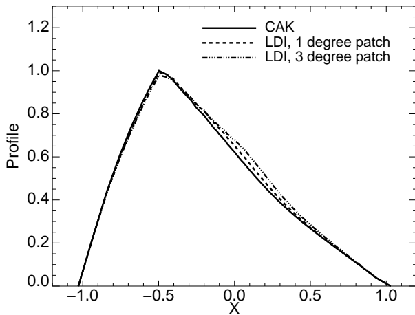
Figure 6. Line profiles for \tau_* = 2.5 , calculated from a smooth CAK model and structured LDI models with patch sizes 1 and 3 degrees (see text), as labelled.
