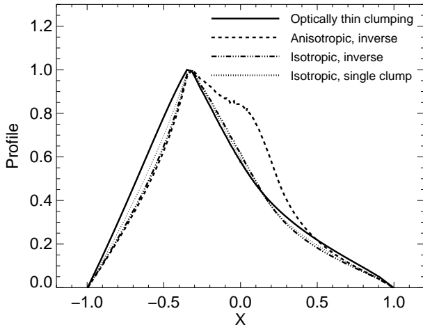
Figure 5. Line profiles for h_\infty = R_* and \tau_* = 2.5 , using different effective opacity laws, as labelled.
